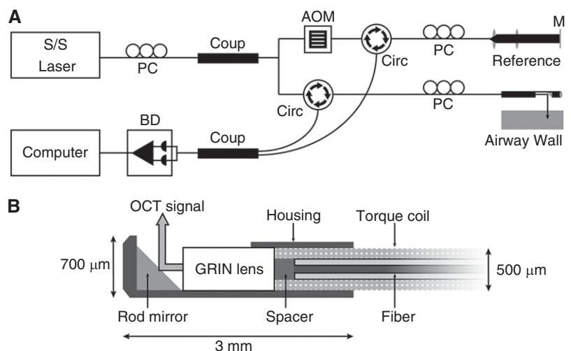
Figure 2. Schematics of long-range optical coherence tomography (OCT) system (A) and cross-section of the distal cap of a 0.7-mm outer diameter scanning probe (B). AOM = acousto-optic modulator; BD = balance detector; Circ = circulator; Coup = coupler; GRIN = gradient refractive index; M = mirror; PC = polarization controller; S/S = swept source.
