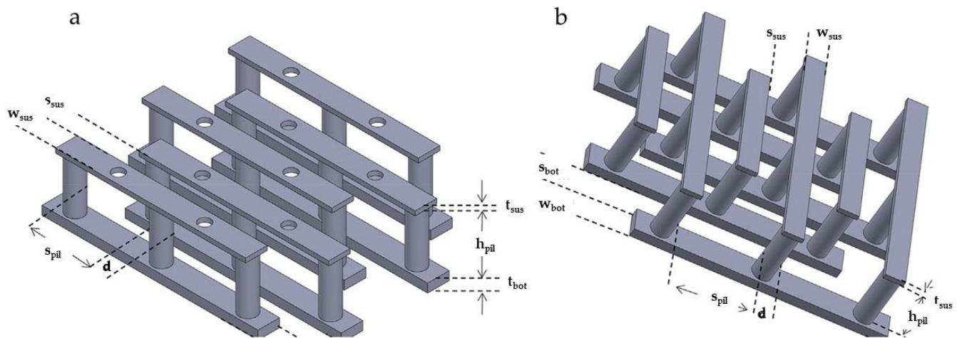
Figure 6. Suspended layer with: (a) stripes connecting pillars of the same finger ( 3D// ); and (b) stripes connecting different fingers of the same electrode ( 3D_{\#} ). Reproduced from [145]. Copyright © 2022, Elsevier under the terms of the Creative Common CC-BY license.
