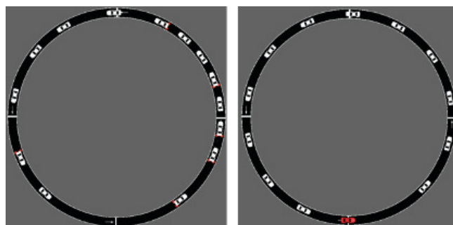
Figure 1 Left: Vehicles not equipped with flow smoothing technology will quickly form stop-and-go traffic waves caused by vehicles braking and then accelerating too much. Right: Introducing a flow-smoothing AV (red car) stabilizes vehicle speeds, primarily by maintaining a gap between the vehicle it is following.
