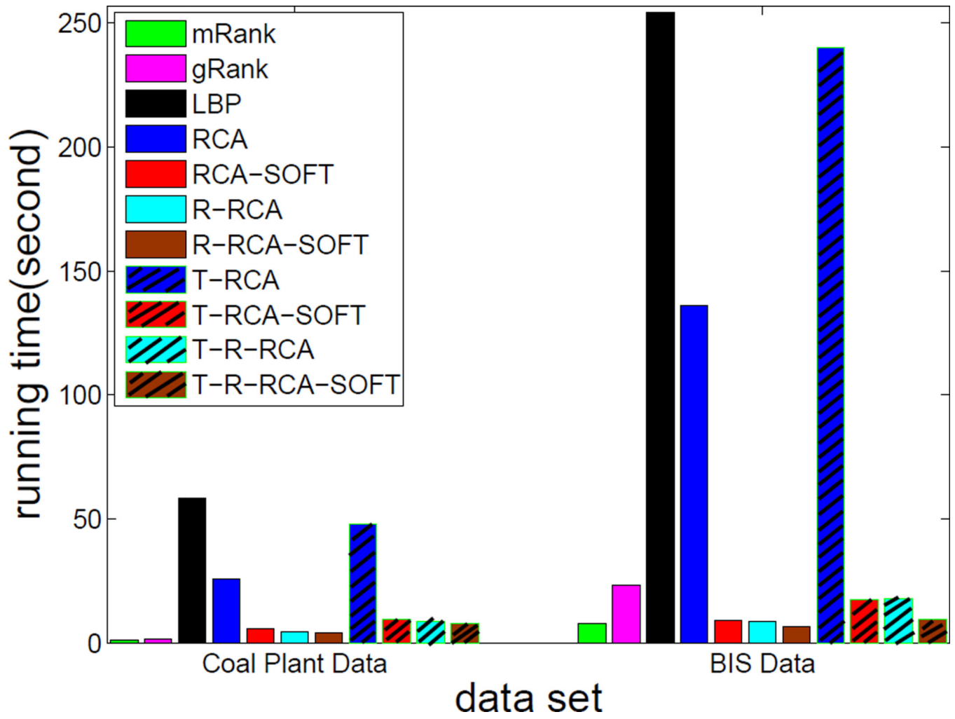
Figure 10. Running time on real data sets.
