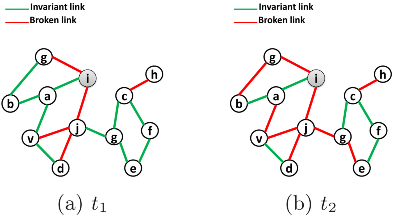
Figure 1. Invariant network and vanishing correlations (red edges).
