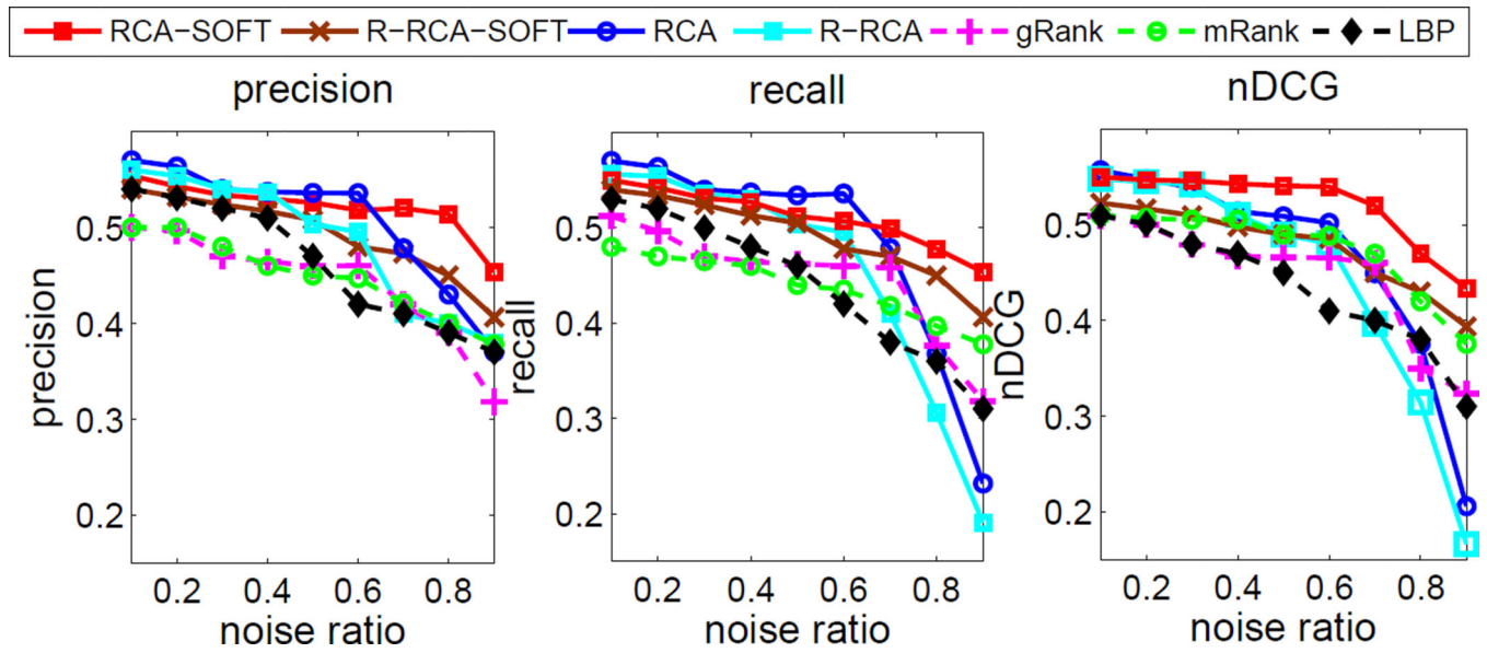
Figure 4. Performance with different noise ratio( K, p = 10 ).
