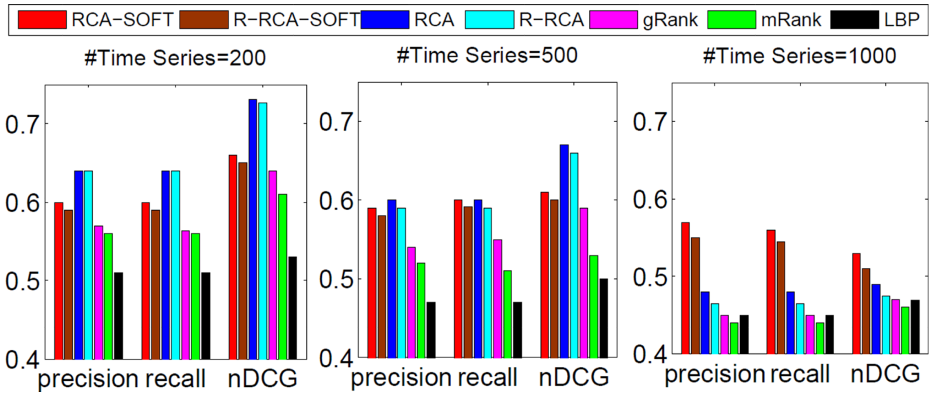
Figure 3. Comparison on synthetic data( K, p = 10 ).
