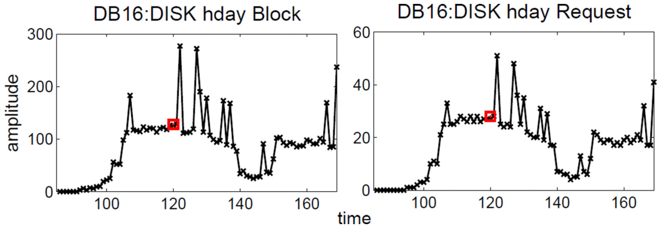
Figure 5. Two example monitoring data of BIS.
