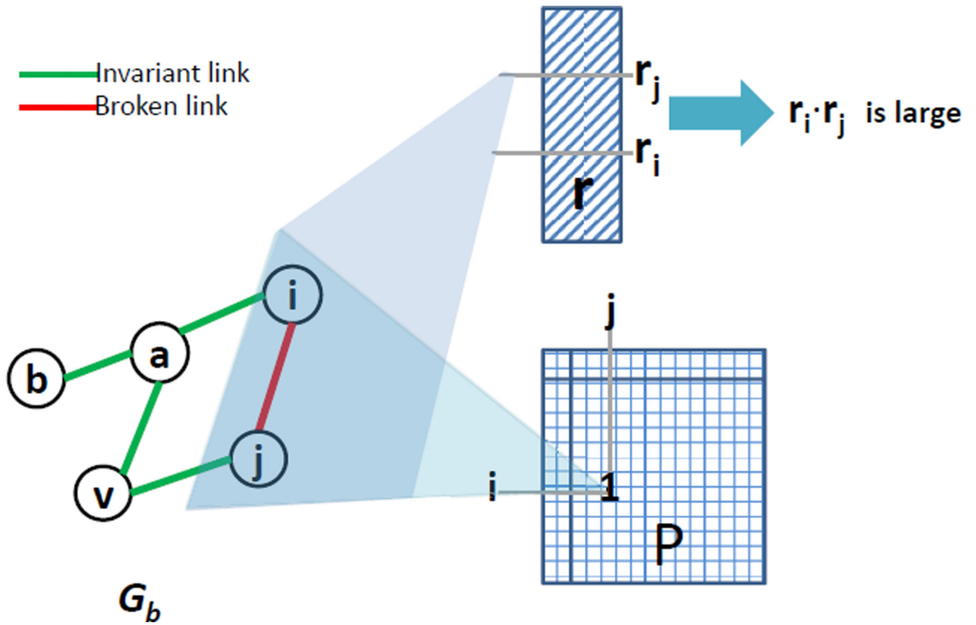
Figure 2. Reconstruction of the broken invariant network using anomaly score vector r .
