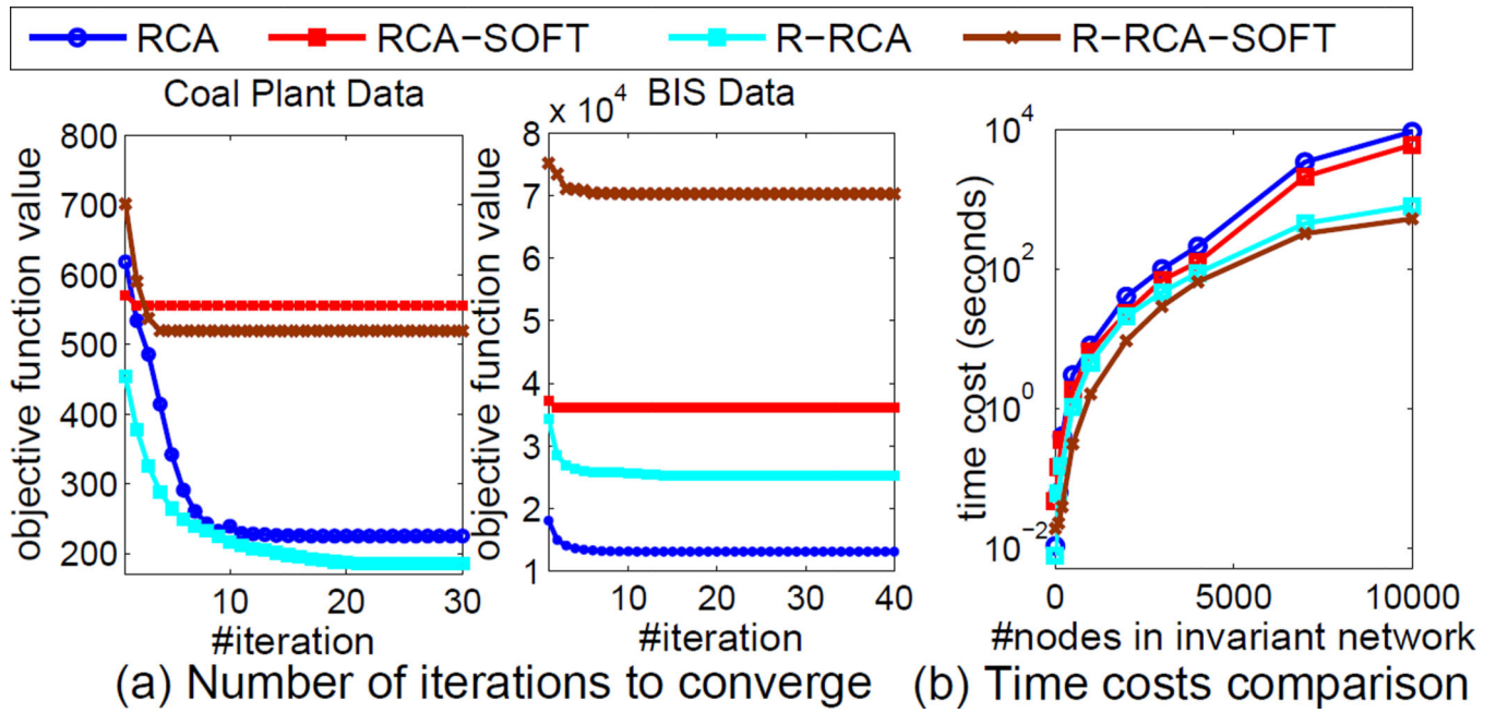
Figure 9. Number of iterations to converge and time cost comparison.
