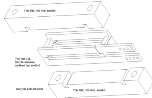
Figure 3: DC dipole magnet, exploded view.
