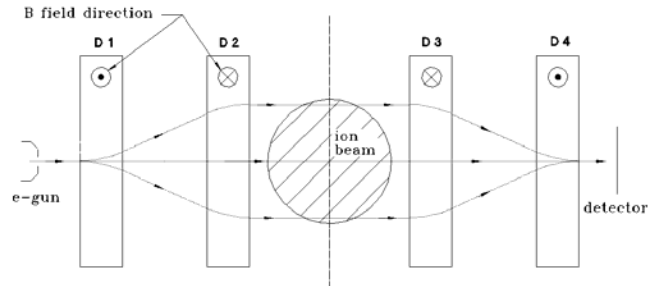
Figure 1: A sketch of non-intercepting beam diagnostic.
