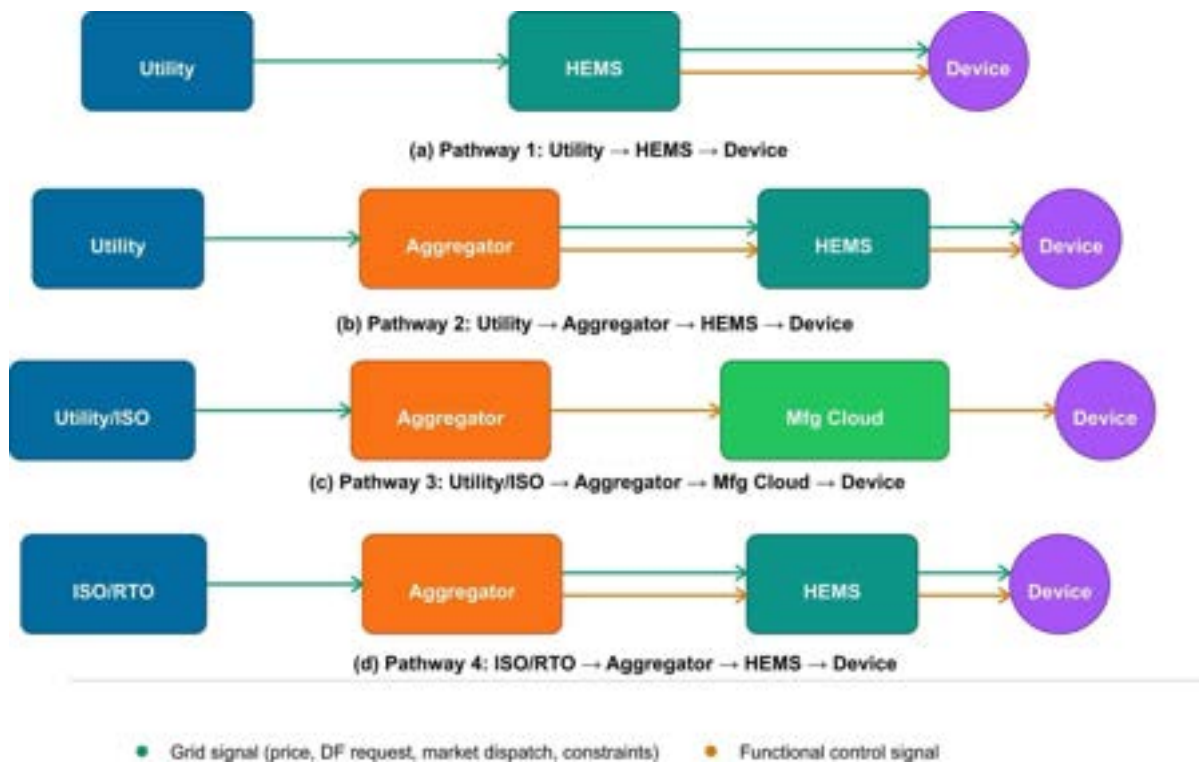
Figure 1. Grid & control communication pathways for residential demand flexibility
