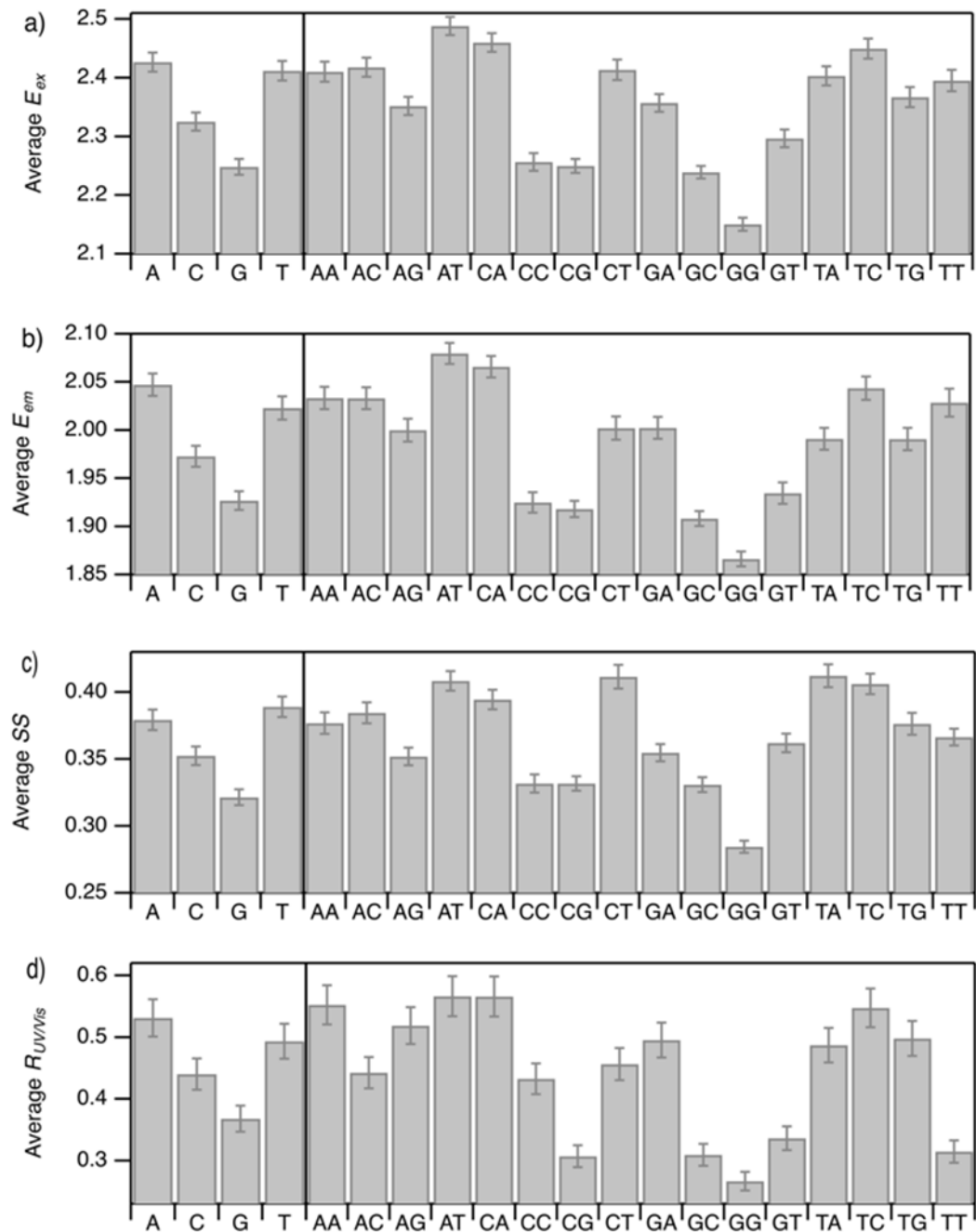
Figure 5: Mean values of (a) E_{ex} , (b) E_{em} , (c) SS , and (d) R_{UV/vis} for each instance of the four nucleobases and the 16 possible two-base motifs in the set of DNA template sequences for the 305 spectrally pure Ag_N -DNAs. Error bars represent standard error, as a measure of precision of the mean.
