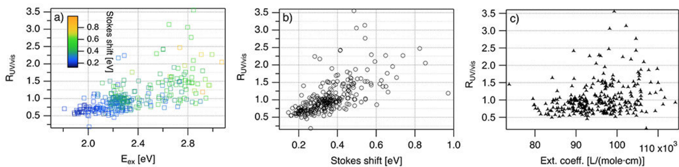
Figure 4: R_{UV/vis} , ratio of areas of UV excitation peak (Region 2) to excitation peak (Region 1), as a function of a) E_{ex} , b) SS , and c) extinction coefficient of the template DNA strand, calculated using the nearest neighbor model. 64,65
