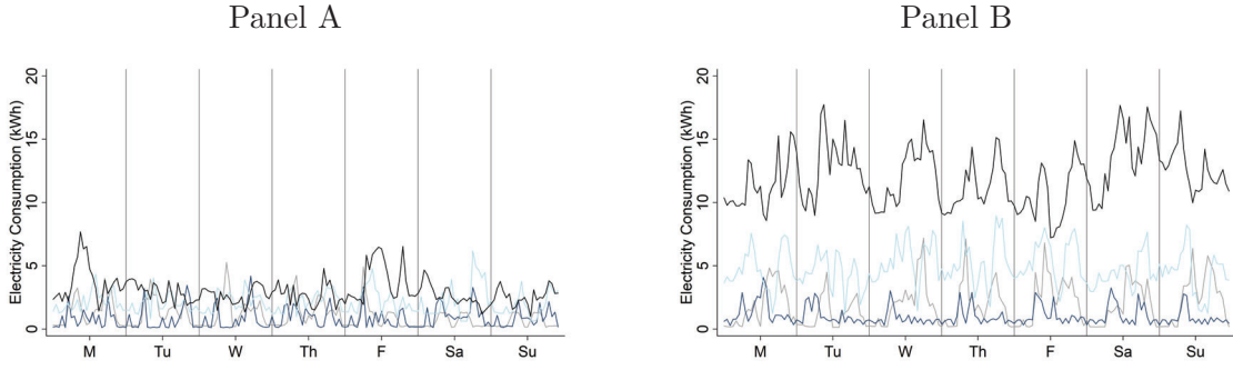
Each panel displays hourly consumption over one week for four randomly selected households. Panel A displays a sample week in summer 2012. Panel B displays a sample week in winter 2010.
