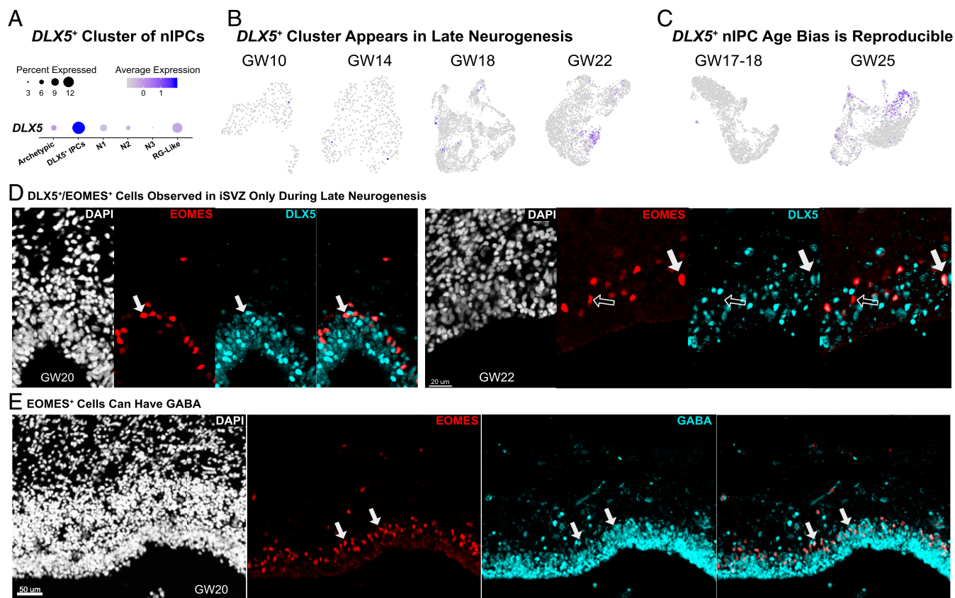
Fig. 5. (A) One cluster of nIPCs expresses DLX5. (B) This DLX5 + cluster appears at later ages in our dataset. The DLX5 + cluster is absent at GW10 and GW14. By GW18, this is a small cluster to the Left , and by GW22, there is a large cluster of DLX5 + cells. This pattern repeats with other datasets. For the GW17–GW18 Polioudakis et al. (16) dataset, a small cluster of DLX5 + cells is visible. (C) Our validation dataset (GW25) confirms a DLX5 + population. (D) DLX5 and EOMES costains a subset of EOMES + cells at GW20 and GW22. Filled-in arrows mark costaining, and empty arrows mark EOMES staining. (E) EOMES + cells at GW20 can also be GABA + , suggesting that inhibitory neurons may be generated from these nIPCs at this time. Colabeled cells are marked with filled-in arrows.
