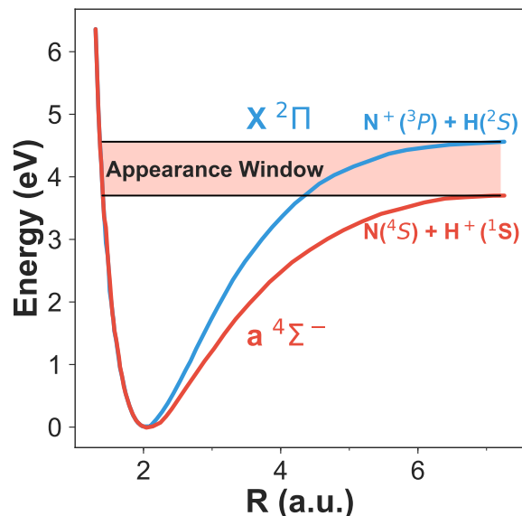
FIG. 9. The potential energy curves for the X^2\Pi ground state and the a^4\Sigma^- state of \text{NH}^+ , extracted from Ref. [40]. Population transfer may occur between these states via spin-orbit coupling, where initially bound excitations on the X^2\Pi state can dissociate on the a^4\Sigma^- state. Only diatomic \text{NH}^+ fragments with internal energy within (or above) the appearance window will dissociate.
