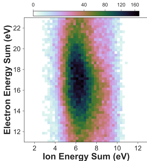
FIG. 10. The yield of N^+ + H^+ after valence PDI of NH_3 as a function of photoelectron pair energy sum and photoion pair energy sum for the ( 1e^{-2} ) ^1E dication state.
