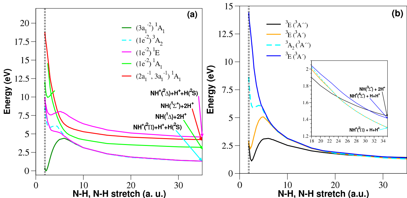
FIG. 1. PES cuts of the \text{NH}_3 dication generated from MRCI calculations as described in the text. Here, two protons are symmetrically stretched while the third remains fixed, with all internal angles frozen at the geometry of neutral ammonia. The zero of energy is set at the ground-state ( ^1A_1 ) of the ammonia dication at the geometry of neutral ammonia, which lies 34.8 eV below the dication [30]. On this energy scale, the 61.5 eV photon energy lies at 26.74 eV. The dashed vertical lines indicate the Franck-Condon region. (a) Cuts of the experimentally identified relevant states; (b) detail of PES cuts for selected \text{NH}_3 dication triplet states. The inset indicates a region of large symmetric stretch distances where charge exchange may occur, as discussed in the text.
