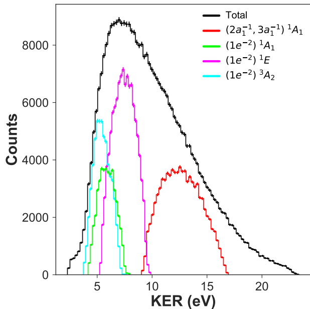
FIG. 6. The yield of \text{H}^+ + \text{H}^+ fragmentation channel of the valence PDI of \text{NH}_3 as a function of KER, shown for the total yield (black), as well as for the four color-coded features corresponding to the identified relevant dication states. The KER distributions for the four features have been scaled by a factor of five, for better visibility.
