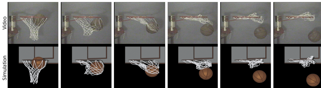
4 Comparison between simulation results for two-way coupling and video footage. The top row of images shows frames captured from video footage of a real basketball and net. The bottom row shows a two-way coupled simulation with matching initial conditions. Images are sampled at 0.067-second intervals.
