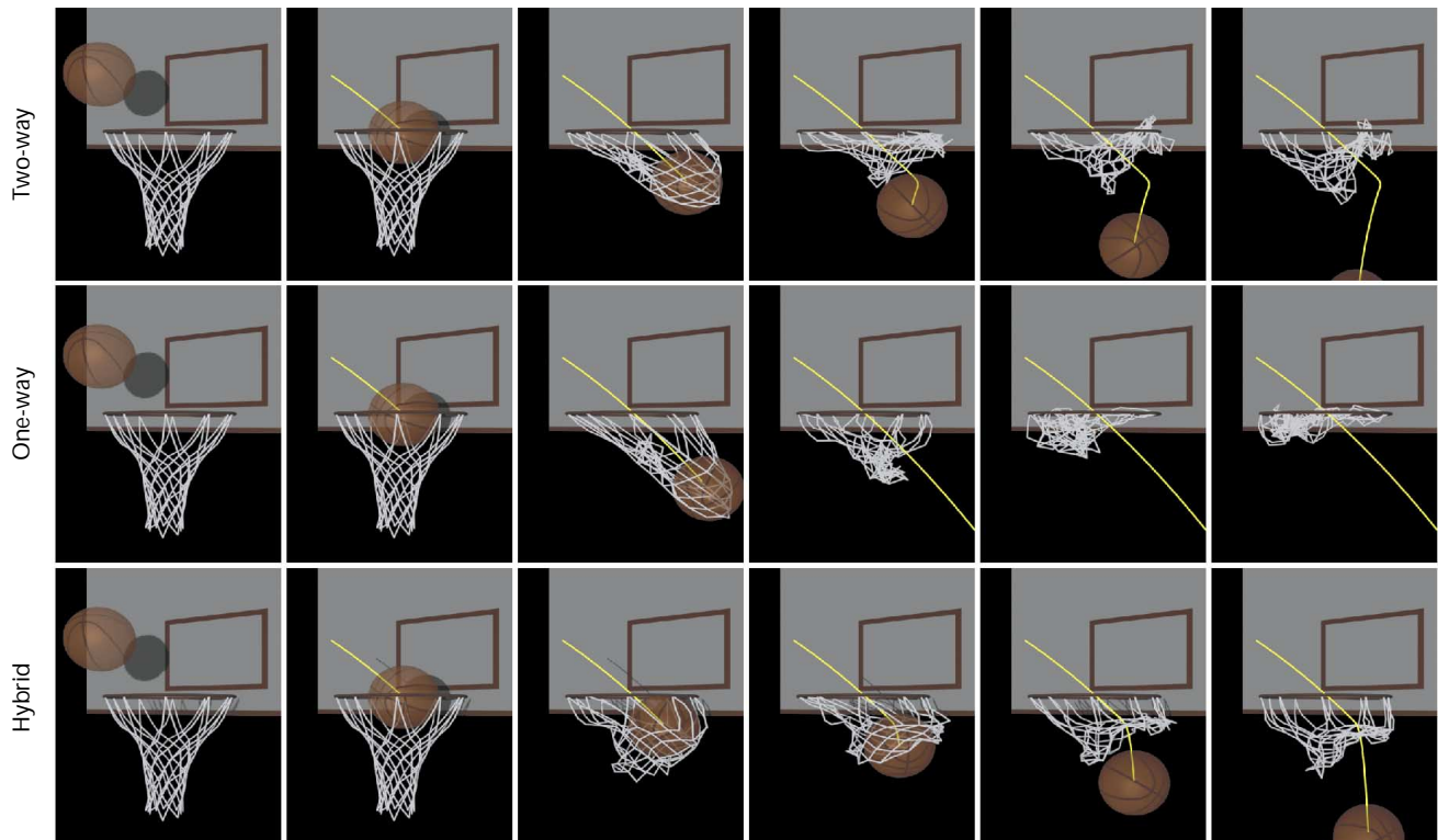
3 Simulated basketball and net with different couplings. The yellow line highlights the path of the ball generated using two-way, one-way, and hybrid coupling. Images are sampled at 0.0833-second intervals.
