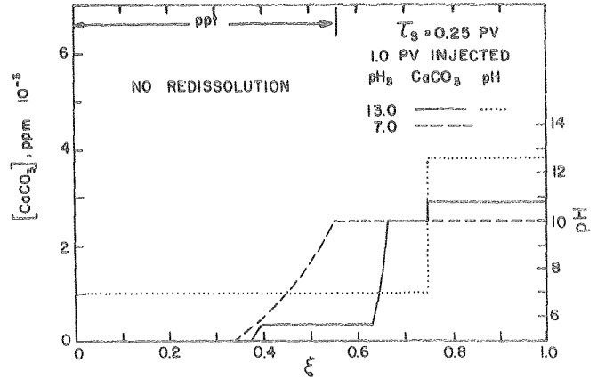
Fig. 26 - Concentration profiles after \tau = 1 PV pulse injection of pH 13.0 and no precipitate redissolution.
