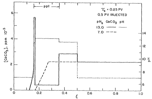
Fig. 28 - Concentration profiles after \tau = 0.5 PV for a 0.25 PV pulse injection of pH 13.0 and equilibrium precipitate redissolution.
