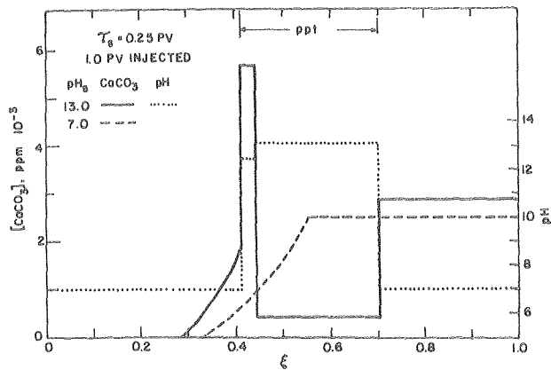
Fig. 29 - Concentration profiles after \tau = 1 PV for 0.25 PV pulse injection of pH 13.0 and equilibrium precipitate redissolution.
