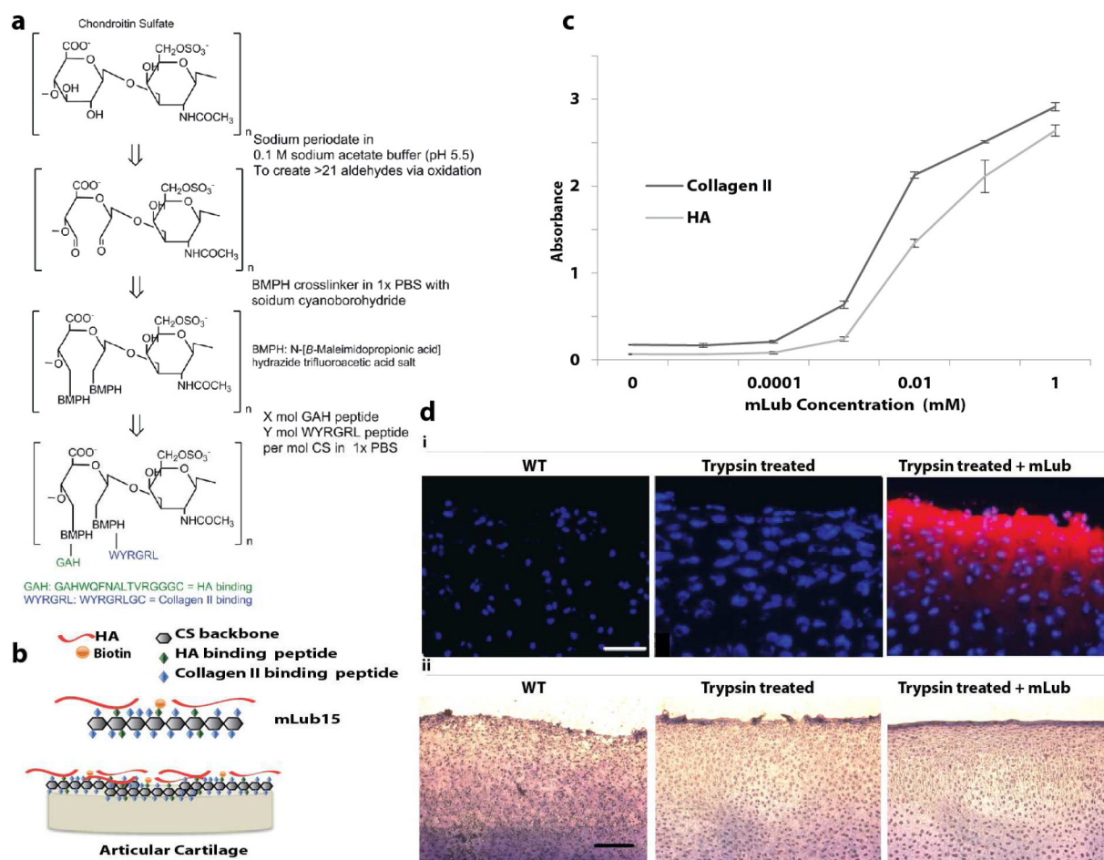
Figure 1. Synthesis of biomimetic lubricin molecule (mLub) bound to type II collagen and HA and spatially localized to cartilage surface
