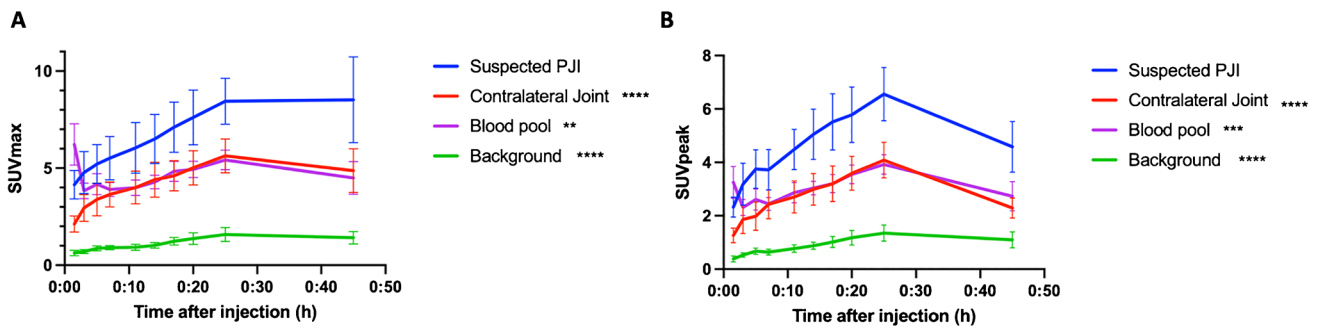
Fig. 4 (A) SUV_{max} and (B) SUV_{peak} time course shows significant difference in D- ^{11}C -Met uptake in joint with suspected infection compared to contra-lateral joint, blood pool, and background. Data represented as mean \pm SEM. ** = p < 0.01 , *** = p < 0.001 , **** = p < 0.0001
