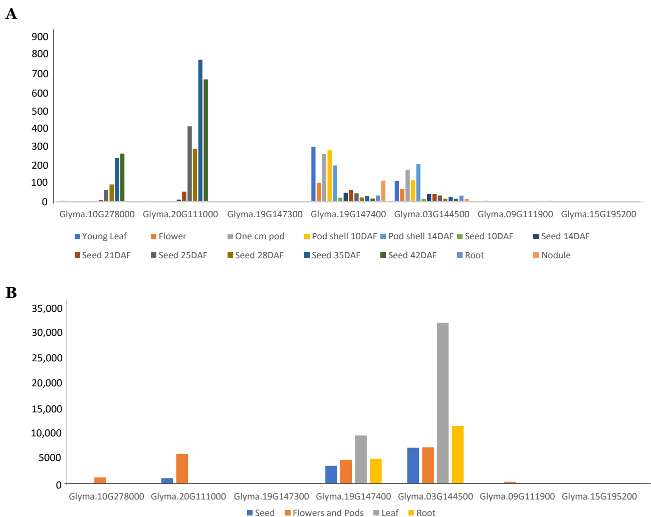
Figure 2. Expression pattern of soybean GmFAD2-1 and GmFAD2-2 gene members. (A) Expression of the seven GmFAD2 members in Williams 82 were retrieved from publicly available RNA-seq data from the SoyBase ( http://www.soybase.org/soyseq ), in addition to (B) the RNAseq data from the cultivar “Forrest”.
