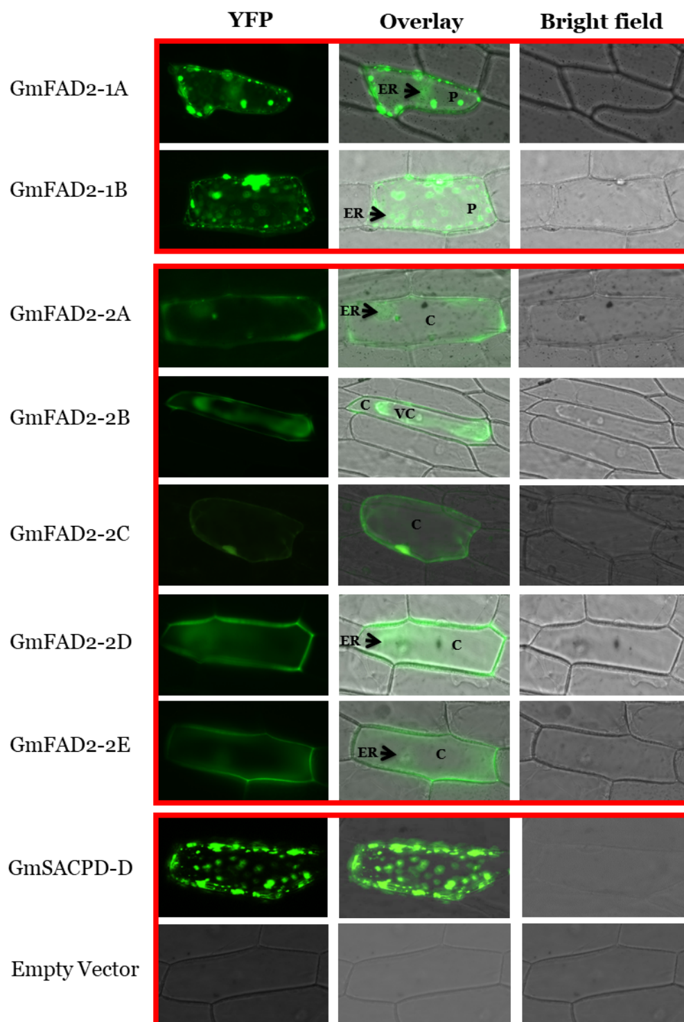
Figure 4. Subcellular localization of soybean GmFAD2-1 and GmFAD2-2 proteins. The GmFAD2 coding sequences from all seven members were fused to eYFP and delivered into onion epidermal cells using biolistic bombardment. GmFAD2-1A and GmFAD2-1B showed an endoplasmic reticulum (ER) and chloroplastic (P) localization pattern. GmFAD2-2A, GmFAD2-2D, and GmFAD2-2E showed a reticulum endoplasmic and cytosol (C) localization. GmFAD2-2C signal was found in the cytosol only. GmFAD2-2B shows a vacuole (VC) and cytoplasmic localization. The chloroplast-targeted GmSACPD-D was used as positive control [29]. Bar = 100 \mu M.
