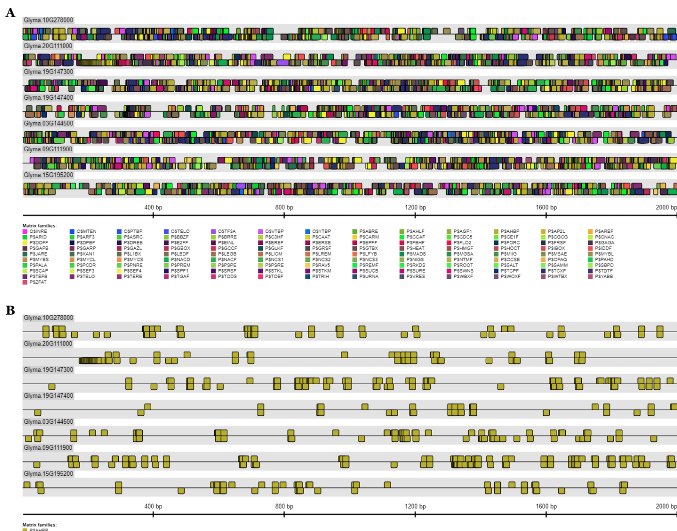
Figure 5. Analysis of putative cis -elements in the promoter region of the GmFAD2-1 and GmFAD2-2 gene members. (A) All identified cis -elements at the GmFAD2-1 and GmFAD2-2 promoter region (–2 Kb upstream). (B) Shows the conserved Arabidopsis homeobox protein domain (P$AHBP) that was shared between all GmFAD2-1 and GmFAD2-2 subfamily members with a total match that was significantly higher (459) when compared to the other cis -elements shown in (A) .
