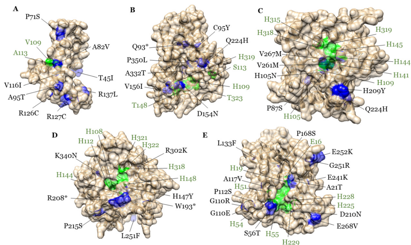
Figure 3. Homology modeling of the five GmFAD2-2 proteins and corresponding identified EMS mutations. Mutated residues on the five GmFAD2-2 proteins identified by Tilling-by-Sequencing + were mapped on the five GmFAD2-2 protein homology models. Homology modeling of the GmFAD2-2A (A), GmFAD2-2B (B), GmFAD2-2C (C), GmFAD2-2D (D), and GmFAD2-2E (E) predicted proteins. The identified mutations and corresponding amino acid changes are shown on blue. Putative di-iron binding sites residues and substrate-binding pocket are shown in green.
