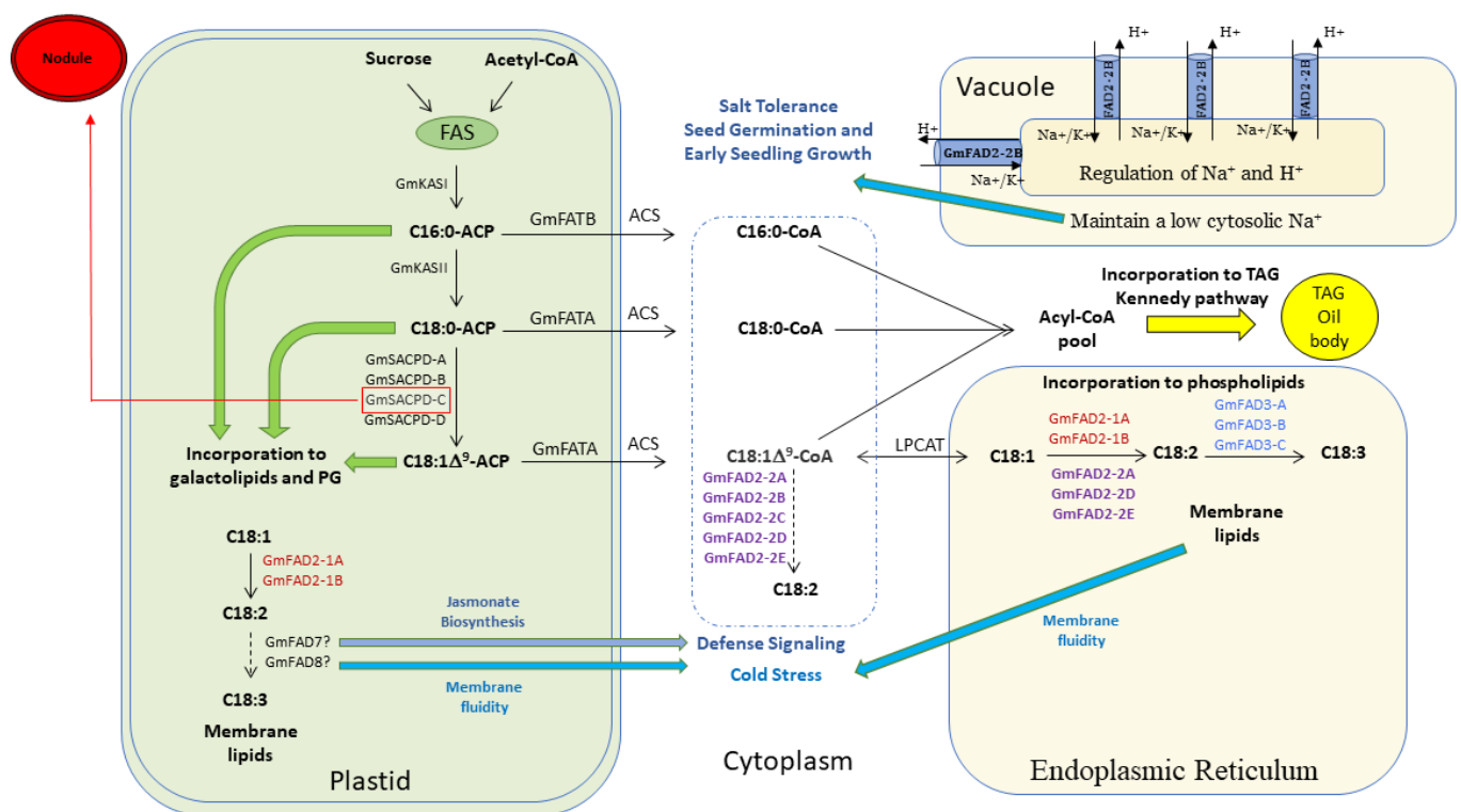
Figure 6. Cartoon deciphering the soybean seed fatty acid biosynthesis pathway. The seven GmFAD2-1 and GmFAD2-2 members are responsible for converting oleic acid (C18:0-ACP) to linoleic acid (C18:1Δ 9 -ACP) in the plastid ( GmFAD2-1A and GmFAD2-1B ), ER ( GmFAD2-1A , GmFAD2-1B , GmFAD2-2A , GmFAD2-2D , and GmFAD2-2E ), and cytoplasm ( GmFAD2-2A , GmFAD2-2B , GmFAD2-2C , GmFAD2-2D , and GmFAD2-2E ). GmFAD2-2B is located in the vacuole and is likely to play a role during seed germination and early seed growth by maintaining low cytosolic Na + as described in Arabidopsis [65]. In bold are the five newly identified fatty acid desaturases involved in the unsaturated fatty acid biosynthesis. GmFAD2-2A , GmFAD2-2B , GmFAD2-2C , GmFAD2-2D , and GmFAD2-2E members present a good alternative for converting oleic acid content without substantially altering the traditional plastidial/ER fatty acid production pathway in soybean. The flux of fatty acids between the plastid and the ER occurs among different plant species [66]. A portion of C16:0-ACP, C18:0-ACP, and C18:1-ACP pool can be incorporated into phosphatidylglycerol (PG) and galactolipids in the plastid. A portion of the acyl-CoA moieties can be incorporated into triacylglycerol (TAG, the major lipid fraction in plant seed oils) biosynthesis in the seed via the Kennedy pathway. GmFAD3 genes are differentially expressed during seed development or cold temperature exposure [67]. The GmFAD7/8 promote C18:3 biosynthesis in the plastid, acting as precursors for the biosynthesis of Jasmonate and are expected to be involved in defense responses and biotic stress signaling [67]. GmSACPD-C is the nodule specific isoforms as shown earlier [29].
