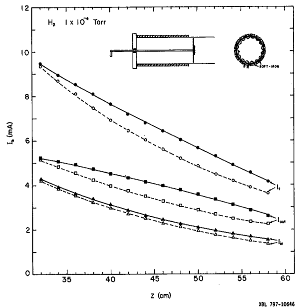
Figure 6. Ion beam current versus collector position with ( \blacktriangle \blacksquare \bullet ) and without ( \triangle \square \circ ) 12 magnet columns on the drift pipe.
