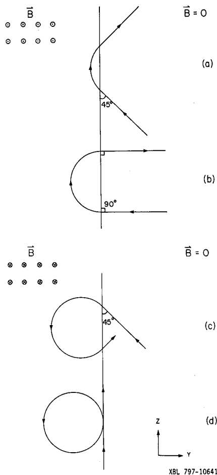
Fig. 1. Reflection of a charged particle by a uniform magnetic field.
