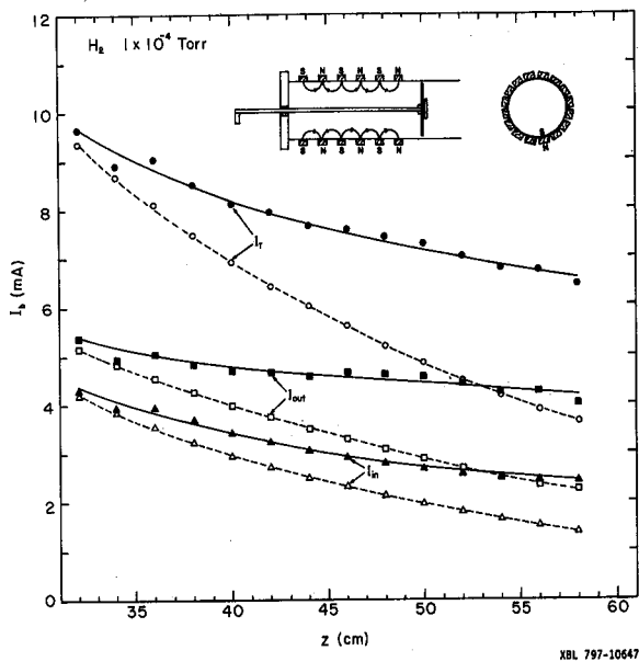
Figure 8. ion beam current versus collector position with (▲■●) and without (△□○) six rings of permanent magnets on the drift pipe.
