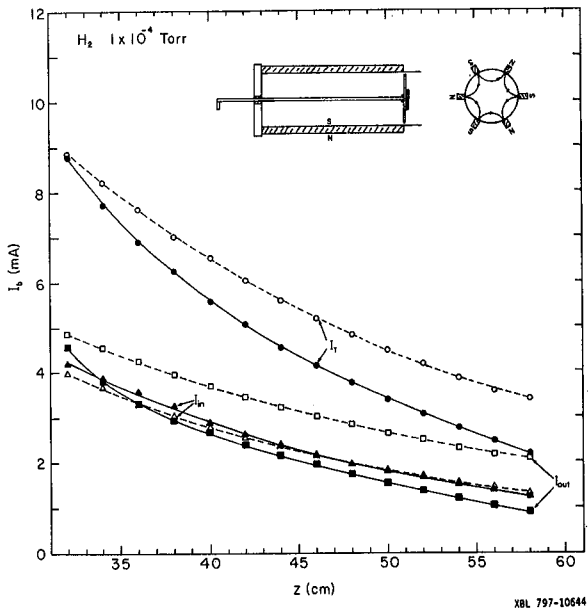
Figure 5. Ion beam current versus collector position with ( \blacktriangle \blacksquare \bullet ) and without ( \triangle \square \circ ) six magnet columns on the drift pipe.
