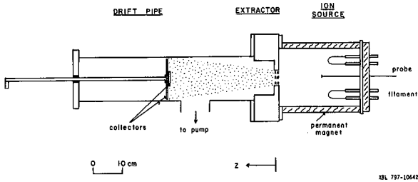
Fig. 3. Schematic diagram of the experimental apparatus.
