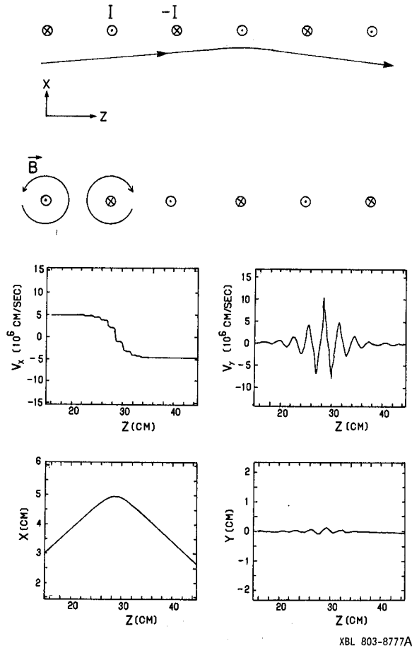
Figure 2. Particle-wire interaction. The velocities v_x and v_y plotted in the computer output are defined in the top figure. The wires are spaced 1 cm apart in z and 10 cm apart in x.
