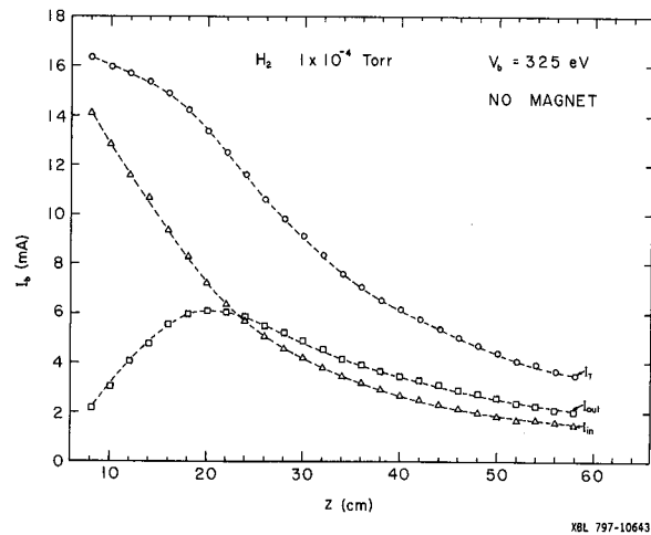
Fig. 4 Ion beam current versus collector position without the presence of permanent magnets on the drift pipe.
