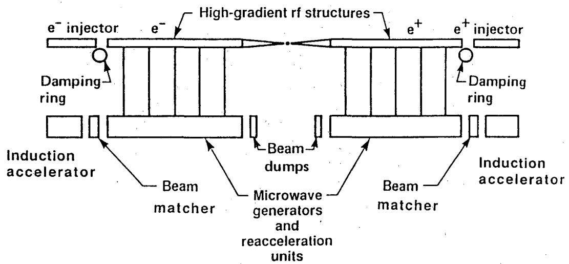
Fig. 8. Schematic of a two-beam accelerator (TBA). The low-energy drive beam provides power to the high-energy ( \approx \text{TeV} ) beam).
