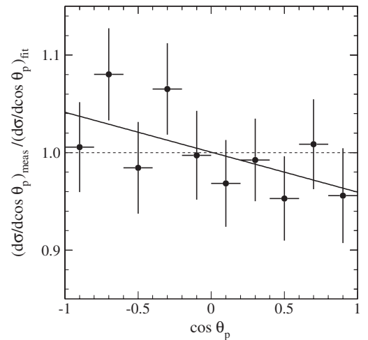
FIG. 11. The ratio of the data distribution from Fig. 10 to the fitted simulated distribution. The line shows the result of a fit of a linear function to the data points.
