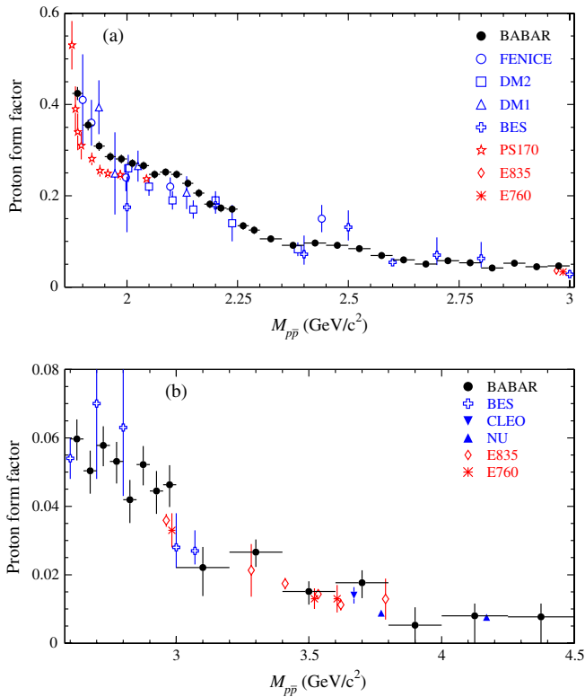
FIG. 16 (color online). The proton effective form factor measured in this analysis, in other e^+e^- experiments, and in p\bar{p} experiments: FENICE [7], DM2 [6], DM1 [5], BES [9], CLEO [10], NU [11], PS170 [12], E835 [14], and E760 [13]: (a) for the mass interval from p\bar{p} threshold to 3.01 \text{GeV}/c^2 , and (b) for p\bar{p} masses from 2.58 to 4.50 \text{GeV}/c^2 .
