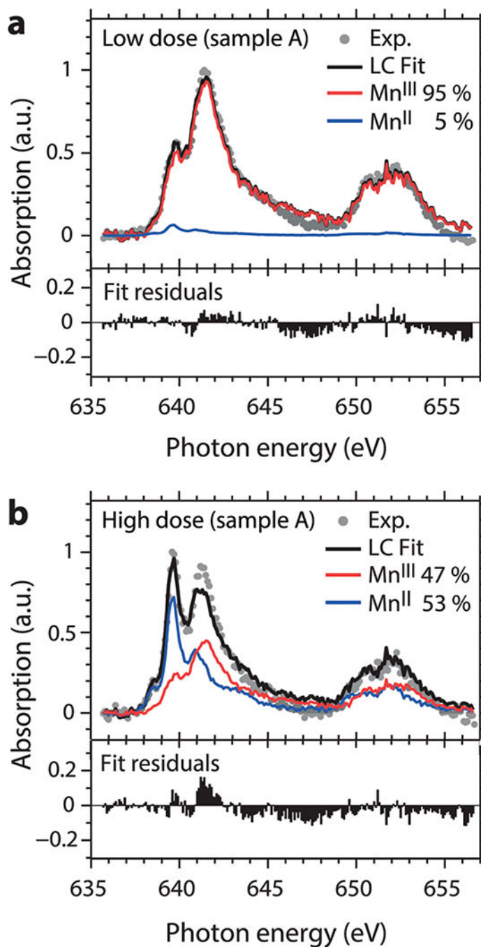
Fig.4. Fits (black) of normalized low-dose (a) and high-dose (b) absorption spectra (circles, taken from Fig. 2a) with linear combinations of damage-free spectra of Mn II (acac) 2 (blue) and Mn III (acac) 3 (red) from ref. 15. Fit residuals are shown in the bottom panels.
