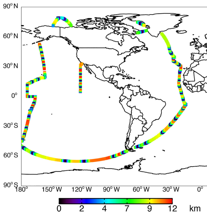
Figure 2. ATom-1 ocean-only flight tracks colored by altitude.
