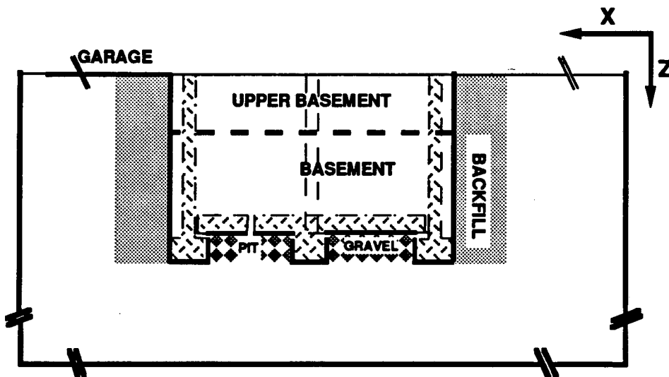
Figure A6d. Cross section A-A of House 002.
