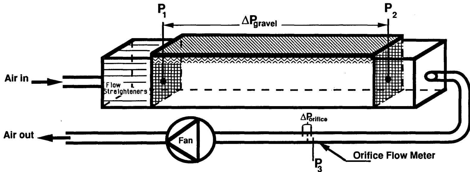
Figure B1. Schematic diagrams of the test apparatus. Low/mid and high/peak velocity data were collected using dry test meters and orifice plate flow meters, respectively, to measure flow rate.
