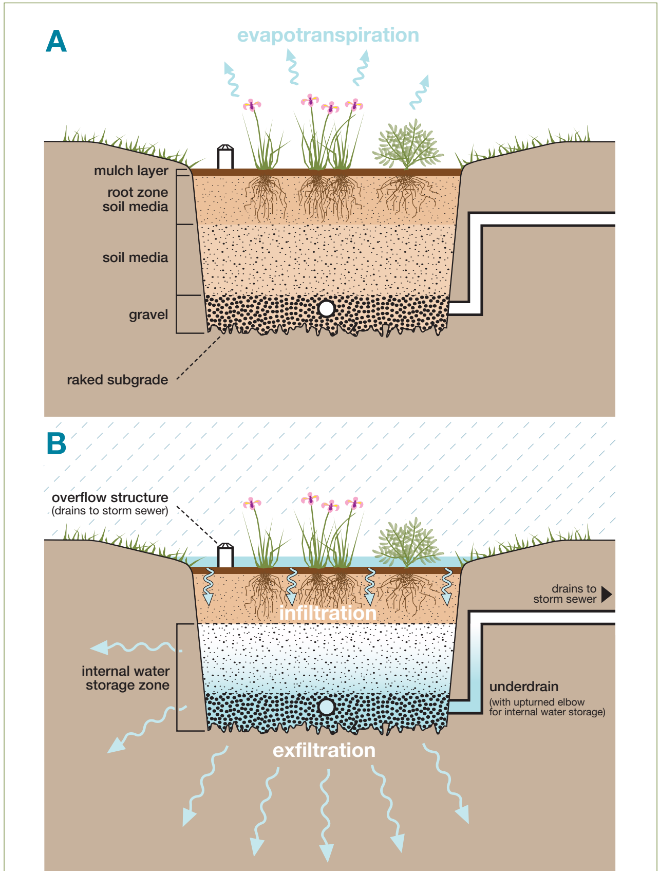
FIGURE 1. Schematic cross section (not to scale) of a bioretention cell, one of the most widely used types of GSI, during (A) dry and (B) wet weather. 33 In this design, water that enters the raised overflow structure remains untreated, but water that flows through the cell and either (1) enters the underdrain or (2) exits (exfiltrates) the cell, moving into (infiltrating) the surrounding soil, has the benefit of treatment. 34
