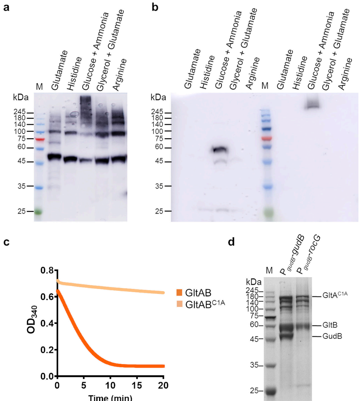
Extended Data Fig. 1. GudB interacts with GltAB
