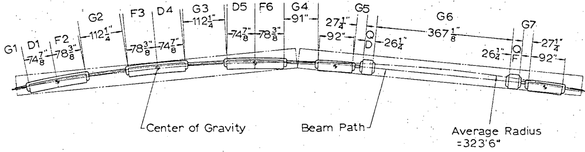
Injector Synchrotron Superperiod
