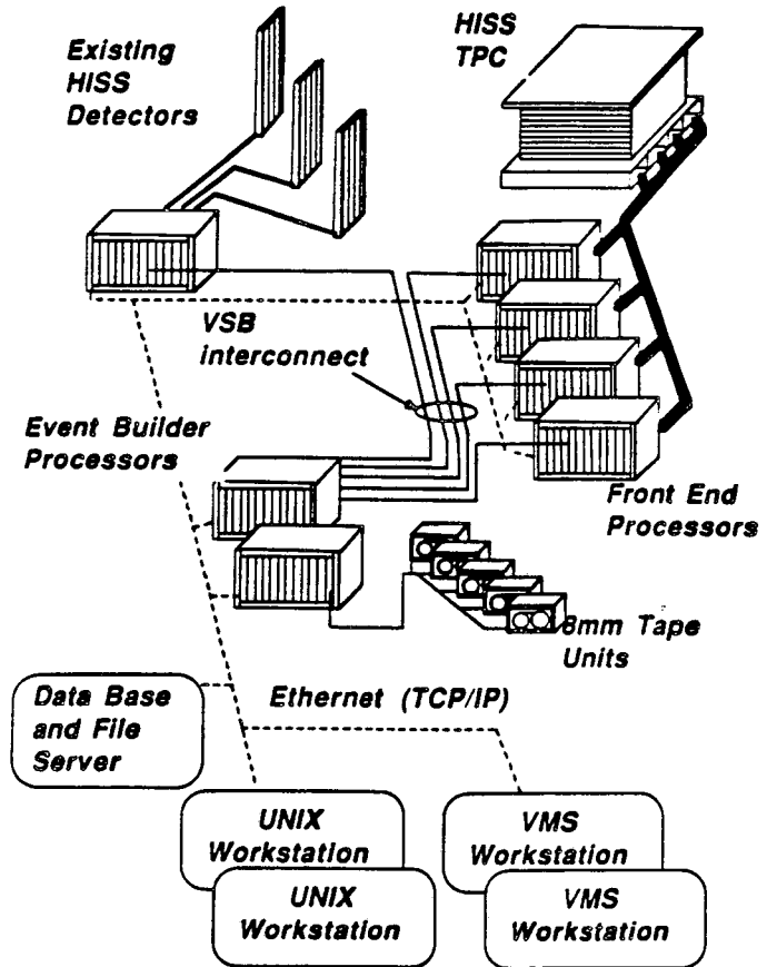
Figure 8: Data acquisition system hardware overview
