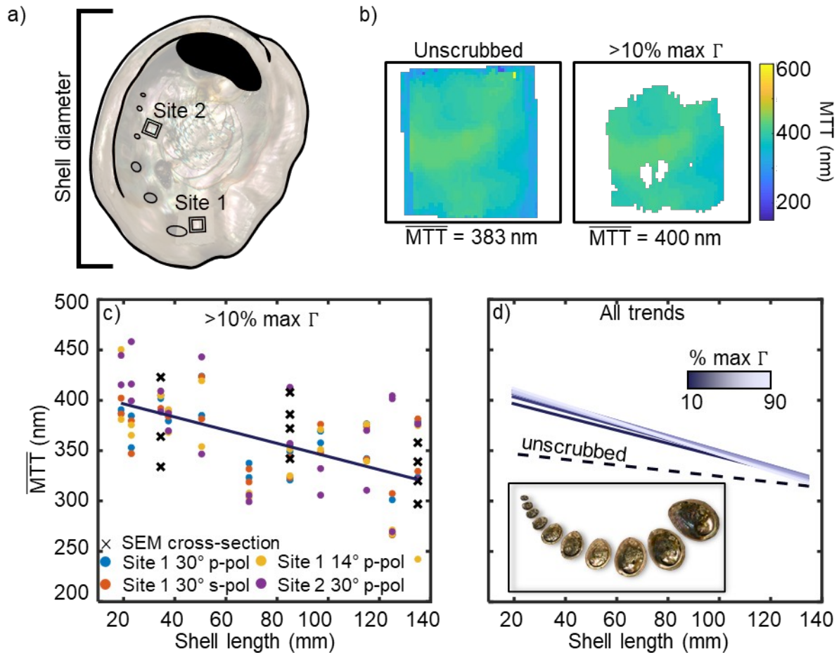
Figure 4: Ontogenetic dependence of red abalone nacre. (a) Two square measurement sites were defined on each of the 22 shells (11 pairs), each 5 mm \times 5 mm. Site 1 was near the outer-most complete gill hole in each shell and contains nacre predominantly formed when the mollusk is older. Site 2 was near the fourth gill hole inward from site 1 and contains nacre formed both when the mollusk was younger and older. (b) Mean tablet thickness (MTT) maps representing a single site on one of the shells. This region is a subset of the full 512 \times 512 pixel map. (c) Plots of all site averages versus shell lengths, with the \Gamma threshold set at 10%. Each pair of shells with the same shell length has 8 thickness measurements in total, with different polarizations and incidence angles, as described in the legend at the bottom of the plot. The dark line is a linear fit to all data points. (d) Plots of linear-fit trends obtained selecting different scrubbing thresholds, with the dashed line representing
