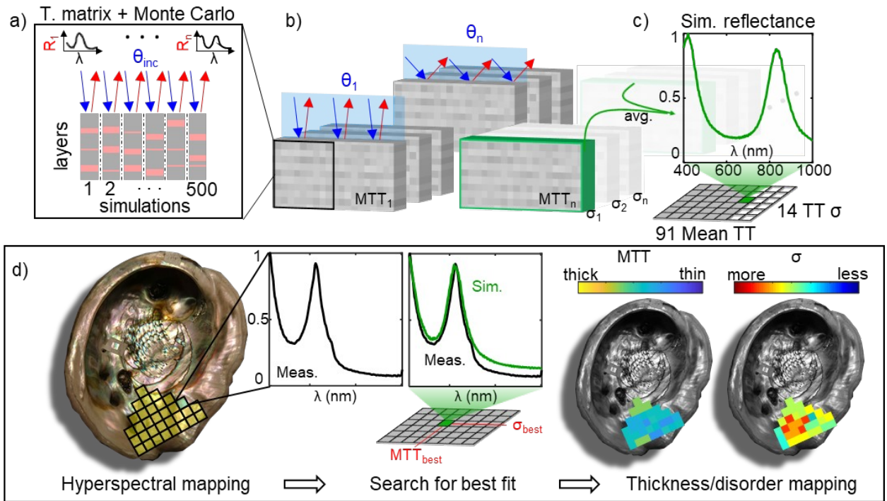
Figure 2: (a-c) Generating simulated reflectance spectra for a given mean tablet thickness (MTT) and tablet degree of disorder ( \sigma ). To generate a single simulated spectrum for a particular MTT and TT \sigma , shown in (c), a Monte Carlo method was used. (a, b) We calculated the reflectance of hundreds of randomly generated thin-film assemblies representing potential nacre layer configurations using the transfer-matrix method at various angles of incidence ( \theta_n ) present within the acceptance angle of our camera. Thousands of simulation results were averaged to produce a single reflectance spectrum, with the peak value normalized to unity. The MTT in our simulation ranged from 150 to 600 nm, with \sigma ranging from 5 to 70 nm. (d) A pictorial overview of the fitting method to extract tablet thickness and \sigma from measured data. Left to right: hyperspectral mapping is performed over a large region of the shell using the setup described in Fig. 1. Each pixel of the spectral map, exaggerated as yellow squares overlaid on the left image, contains a full reflectance spectrum spanning 400-1000 nm, here normalized to unity. Measured data at each pixel were then compared to every simulated spectrum generated from (c) until the lowest mean squared error was found. Each pixel was then assigned the best-fit tablet thickness ( MTT_{best} ) and disorder ( \sigma_{best} ) to generate maps of nacre tablet thickness across the entire analyzed region. Note that the maps in (d) are schematics and do not represent a physical measurement.
