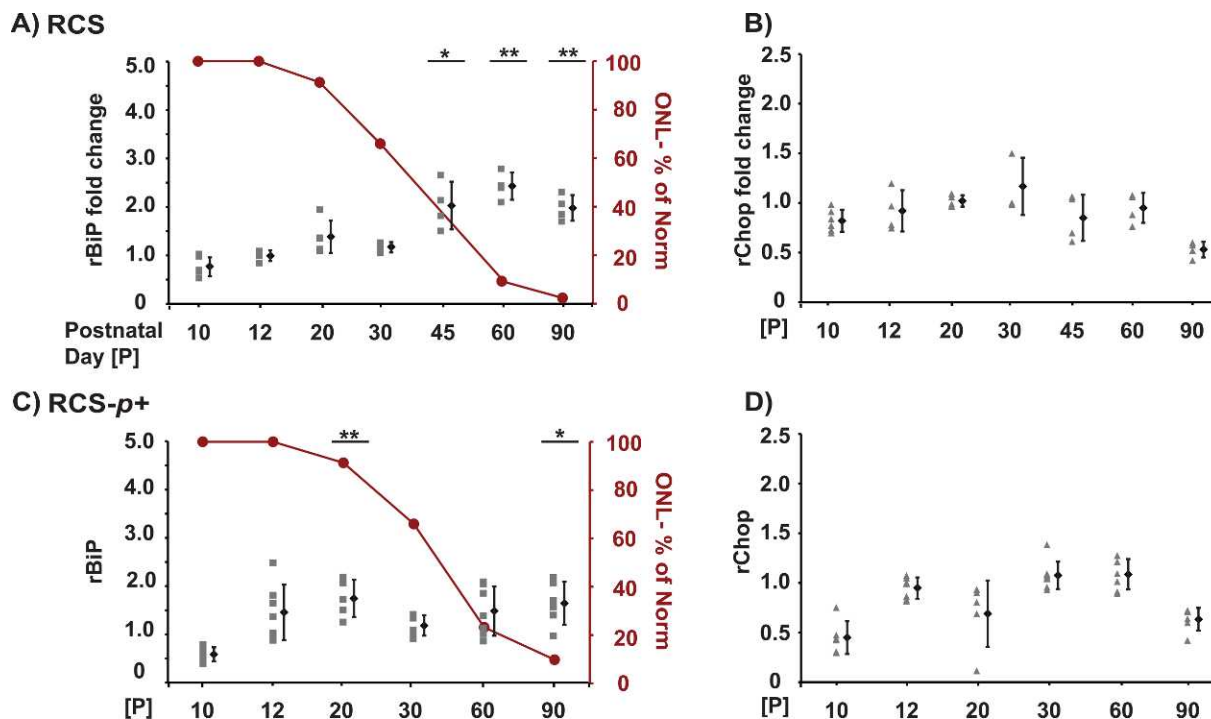
FIGURE 3. Induction of BiP and Chop in retinas of RCS rats. Analysis of BiP and Chop mRNA levels by quantitative PCR using rat retinas at indicated postnatal day ages (P). Samples were plotted relative to average of gene levels of wild-type RCS- rdy + control animals at the same age. (A) BiP and (B) Chop mRNA levels of RCS animals. (C) BiP and (D) Chop mRNA levels of RCS- p + animals. (A–D) Retinas from three to eight animals were collected for each postnatal day age, and the gene expression level from each animal is plotted individually to the right. The mean value and SD for the cohort of animals at each time point are plotted to the right. The amount of degeneration is graphically presented as a percent of the normal ONL thickness at each time point as red line for each animal model (A, C). P values represent the following asterisk system: * P < 0.05, ** P < 0.005.
