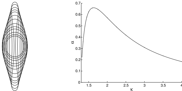
FIGURE 3. Hollow vortices for \delta = -\tau . Left panel: vortex shapes for \kappa = 1.4, 1.5, 1.6, 1.75, 2, 2.25, 2.5, 3, 3.5, 4 ; right panel: nondimensionalized vortex area vs. \kappa .
