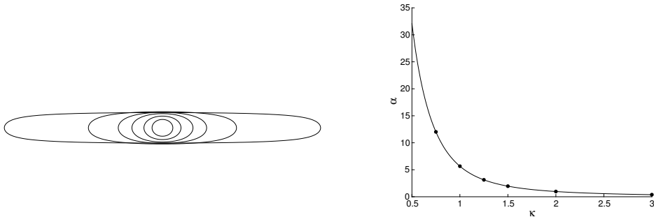
FIGURE 5. Hollow vortices for \delta = \tau . Left panel: vortex shapes for \kappa = 0.75, 1, 1.25, 1.5, 2, 3 ; right panel: nondimensionalized vortex area vs. \kappa .
