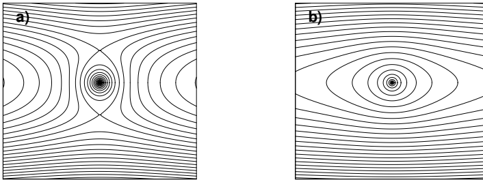
FIGURE 1. Streamline patterns of the point vortex solution: a) \delta = -\tau ; b) \delta = \tau
