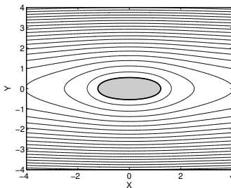
FIGURE 4. Streamline pattern for \delta = \tau and \kappa = 1.5 .
