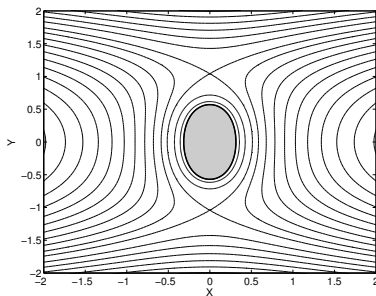
FIGURE 2. Hollow vortex streamlines for \delta = -\tau and \kappa = 2 .
