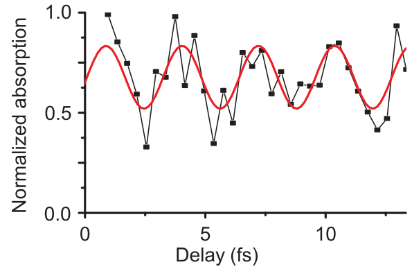
FIG. 3 (color). Presence of oscillation in the signal as a function of arrival time of the readout pulse indicates coherence between the |x+\rangle and |t-\rangle states that is present after the preparatory and selective excitation pulses. The solid red line is the best sinusoid fit to the data points.
