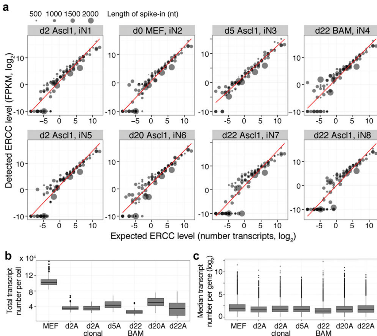
Extended Data Figure 2. Total number of transcripts per cell decreases during MEF-to-iN cell reprogramming
