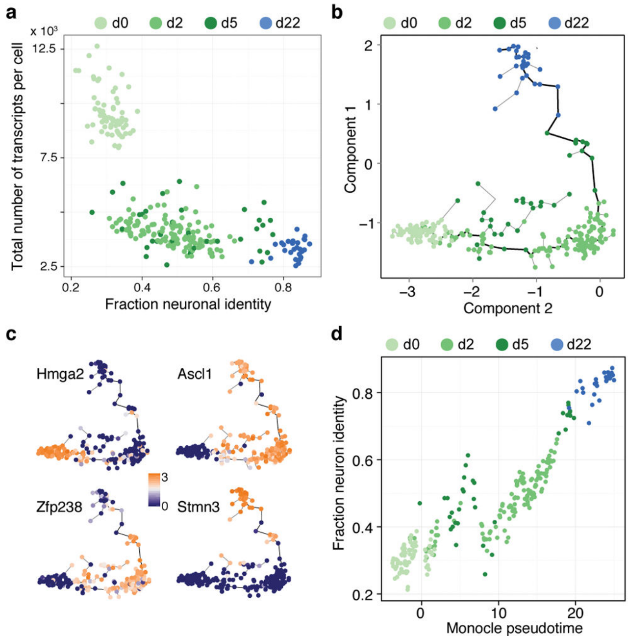
Extended Data Figure 7. Comparison of Monocle and quadratic programming with respect to ordering of neuronal cells through the reprogramming path
