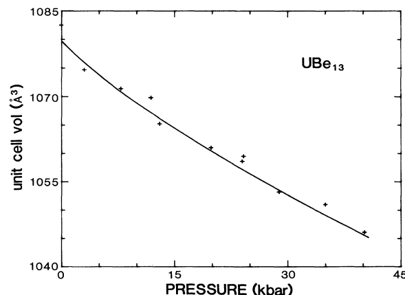
FIG. 1. Volume of the \text{UBe}_{13} unit cell as a function of pressure.
