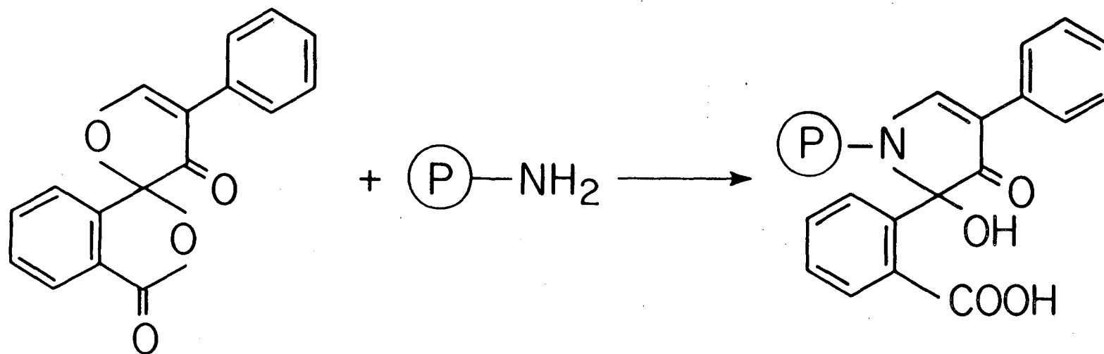
Fluorescamine
