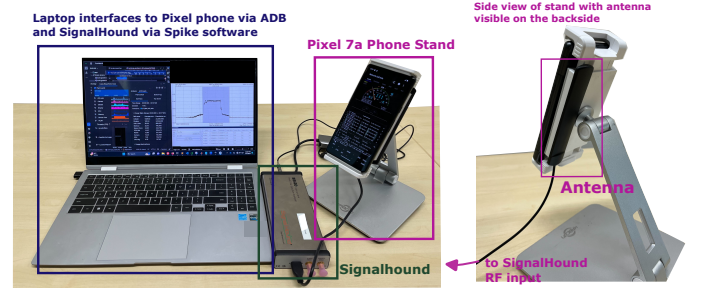
Figure 13: Setup to measure both the transmit power of phone, as well as power consumption reported via ODPM rails
