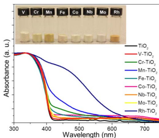
Figure 2. Photograph of various transition-metal doped TiO 2 nanowires and UV-vis spectra of various transition-metal doped TiO 2 nanowires.
