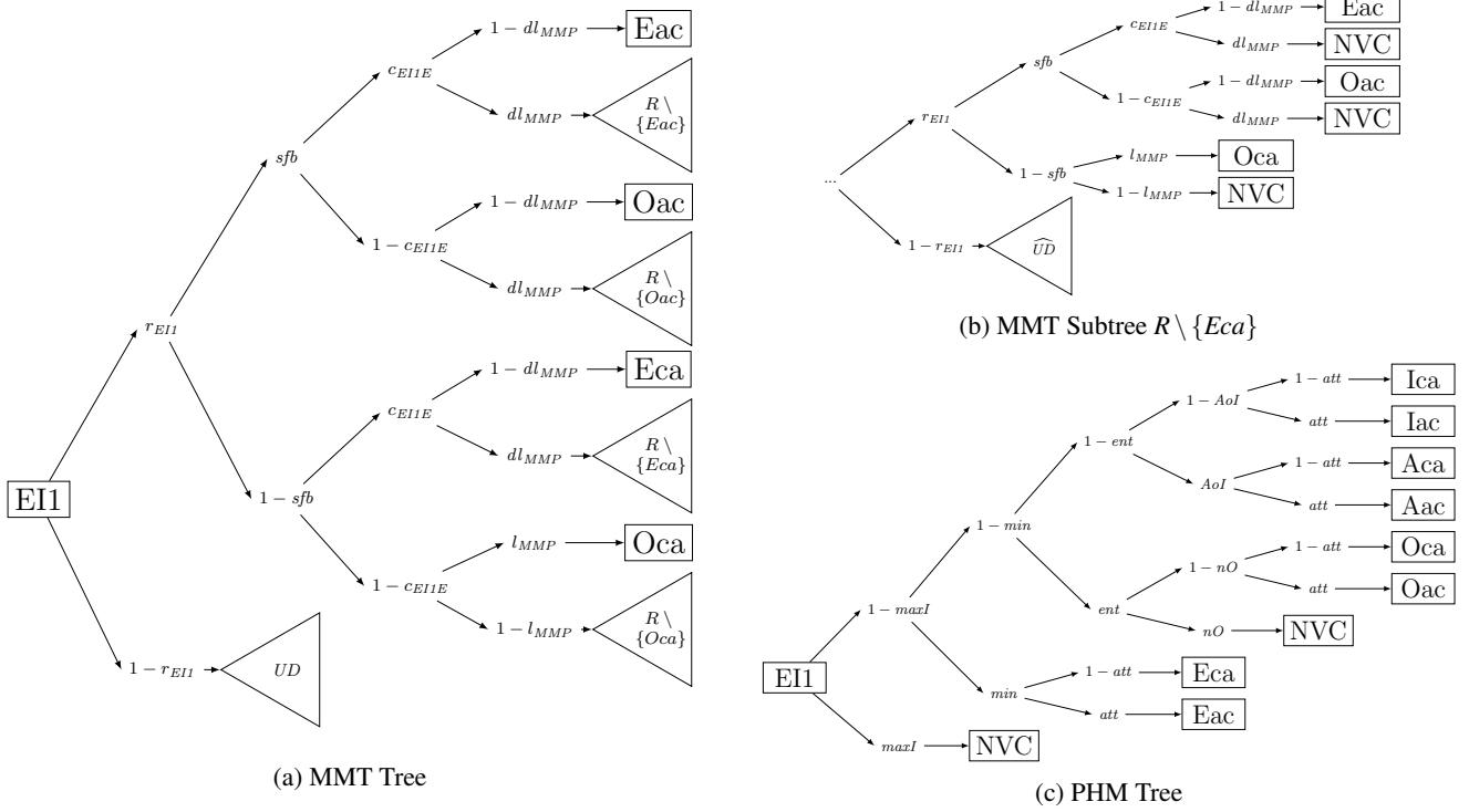
Figure 2: The MMT and PHM trees for “No A are B. Some B are C.” (EI1). Capital letters refer to the quantifiers ( A = All , I = Some , O = Some...not , E = None ). Manifest, observable variables are drawn as squares (on the left: the premises, the number indicates the figure; on the right: responses as conclusions, ac indicates A-C and ca C-A conclusions e.g., Eac = “None of the A is C”; NVC = “no valid conclusion”). In between, the assumed latent states (not observable) are printed borderless. The MMT tree begins with the reasoning parameter r_i ( i = Syllogism), followed by the Figural Bias parameter for applicable syllogisms (e.g., for IE1 the Strong Figural Bias sfb ), and (if necessary) the decision between the predicted quantifier (e.g., C_{EI1E} ). Finally, the preliminary conclusion is confirmed with l_j if correct, with 1 - dl_j otherwise, or rejected with the respective converse probability (here: j = MMP ). After rejecting, a new conclusion is sought (see Figure 2b, subtree: R \setminus \{c\} , with c being the discarded conclusion). UD indicates the uniform distribution over all nine conclusions, \widehat{UD} over the remaining eight. The PHM tree begins with the max-heuristic in the case of max-premise being I ( maxI ), selects quantifier E from min-heuristic ( min ), or quantifier O from entailment-heuristic ( ent ), or either of the remaining two ( AoI ). In the case of O, the O-heuristic is applied ( nO ). Finally, the order of end terms is set using or refusing the attachment-heuristic ( att ).
