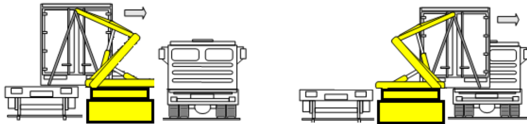
Figure 4-7 Truck-train Transshipment Solution 2: Side Loading Using Flexible Crane Mounted on Rail on the Platform
