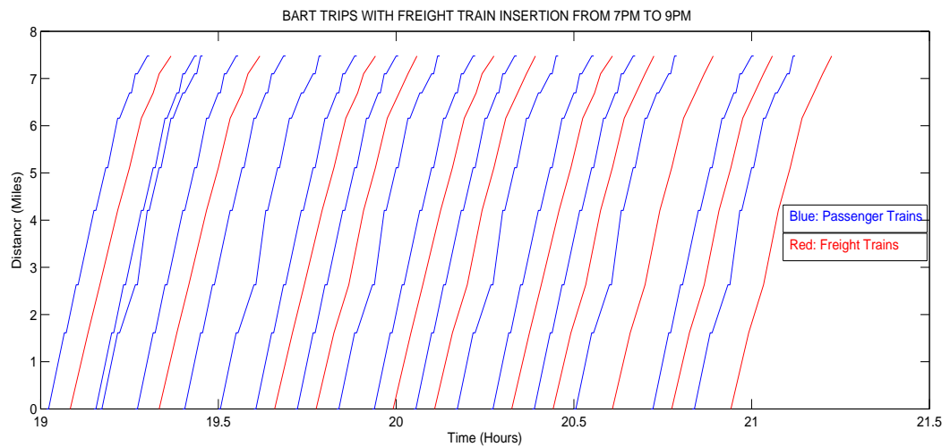
Figure 3-12: Time Space Diagram for Freight train insertion in the evening slots
