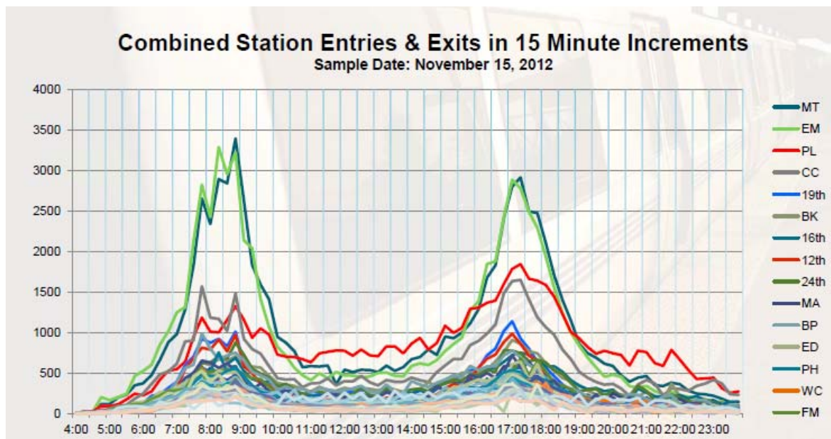
Figure 4-1: BART system load for Transbay Lines
