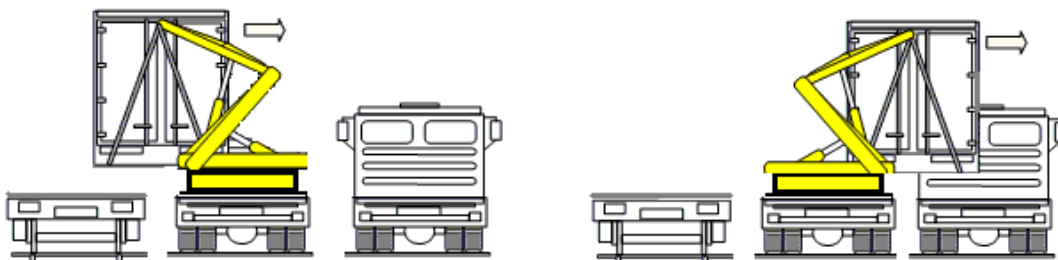
Figure 4-8 Truck-train Transshipment Solution 3: Side loading using a flexible crane on a heavy-duty-vehicle
