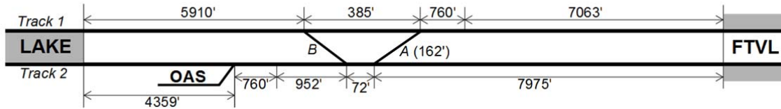
Figure 3-3: Rail Track Geometry at Access Point to Oakland Annex Shop (OAS) for section between Fruitvale (FTVL) and Lake Merritt (LAKE)
