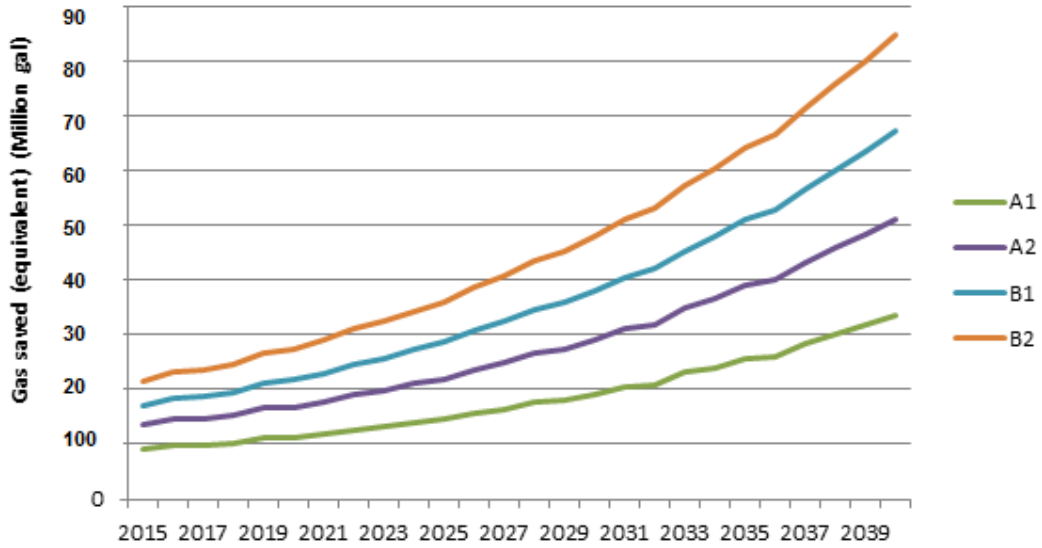
Figure 4-9. Predicted annual Gas (Million Gal) saving vs. Status Quo for the 4 alternatives
