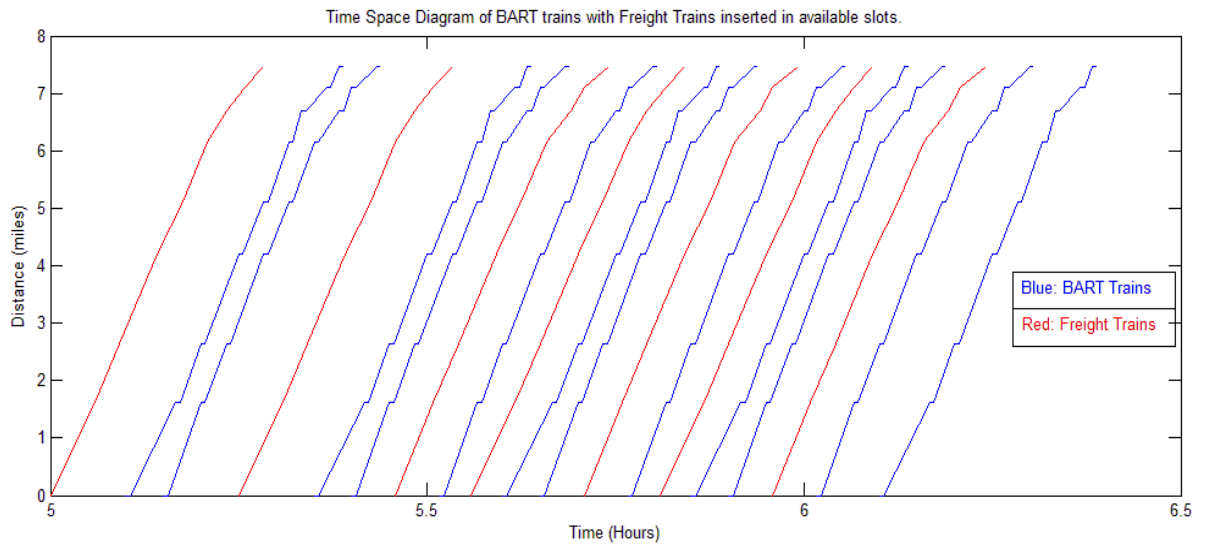
Figure 3-11: Time Space Diagram showing Freight train insertion in the morning slots
