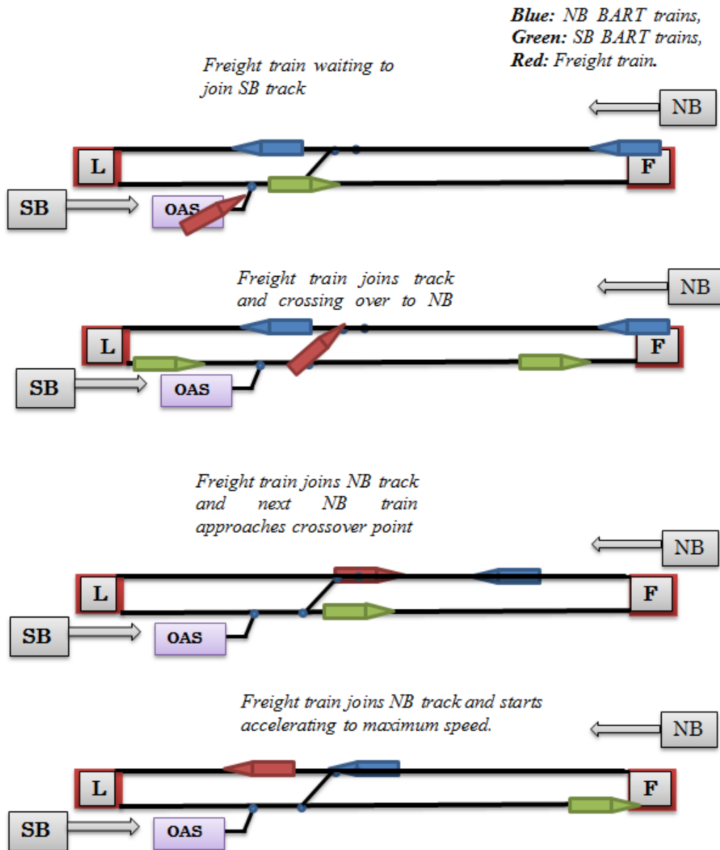
Illustration of Northbound insertion between Fruitvale and Lake Merritt BART station:
