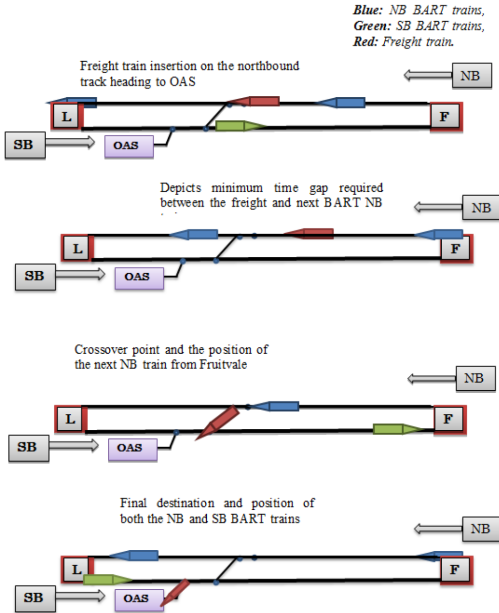
Figure 3-6: Illustration of a NB freight train movement into OAS
