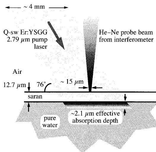
Fig. 7. Expanded view of Er:YSGG irradiation of saran covered water samples (not to scale).
