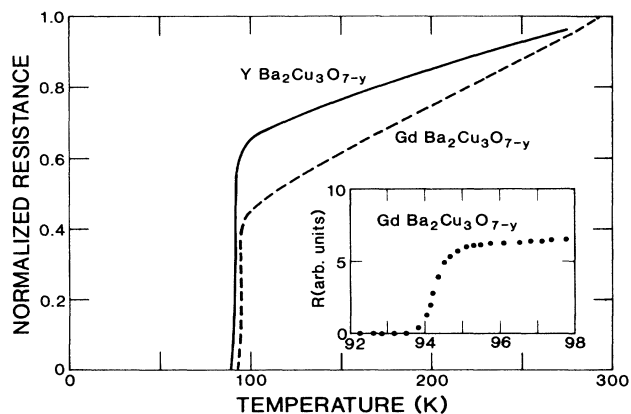
FIG. 1. Resistance, normalized by its value at 300 K, as a function of temperature for YBa_2Cu_3O_{7-y} and GdBa_2Cu_3O_{7-y} . Typical values for the resistivity of both samples at room temperature are 500 \mu\Omega \text{ cm} or greater. Higher values for the resistivity are found in less-well-sintered specimens. The inset shows a rather sharp phase transition ( \Delta T_c = 0.6 K).
