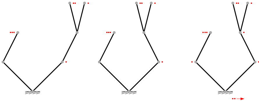
Fig. 3 Three examples of fully parked trees. Notice that the first two have no outgoing flux and represent the same plane tree but their embeddings in \mathbb{B} is different. The last fully parked tree on the right has an outgoing flux of 2 cars
