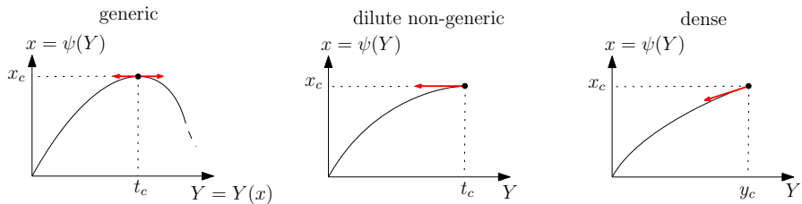
Fig. 5 Illustration of the three scenarios for the change of variable x \mapsto Y(x) . Our standing assumption (\star) holds in the first two cases
