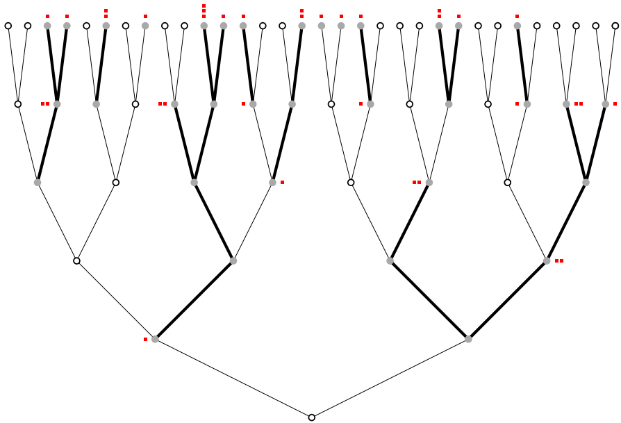
Fig. 2 Illustration of the parking process in the first 5 levels of the full binary tree. The car arrivals are represented by red squares (including the cars that may come from higher levels on top of the tree). After the parking process, the vertices accommodating a car are displayed in gray, whereas the free spots are displayed in white. The connected components of parked cars are drawn with thick lines, they are fully parked trees
