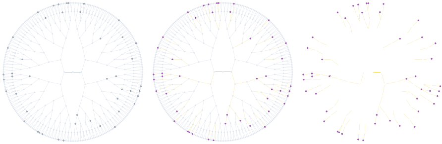
Fig. 1 Simulation of the parking process on the first 9 levels of the full binary tree (the edges are oriented towards the origin of the tree which is at the center of the figures). The dotted vertices on the left figure initially contain 2 cars whereas the others are void. In the middle and right figures, the highlighted edges have seen a positive flux of car
