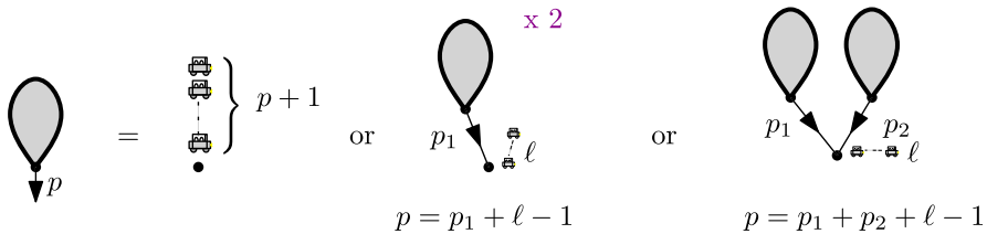
Fig. 4 Illustration of Tutte's recursive decomposition at the root vertex. On the left a fully parked tree with flux p . If n = 1 , then the tree is just a vertex with p + 1 cars arriving on it. Otherwise, it has one or two children which are the root of smaller fully parked tree
