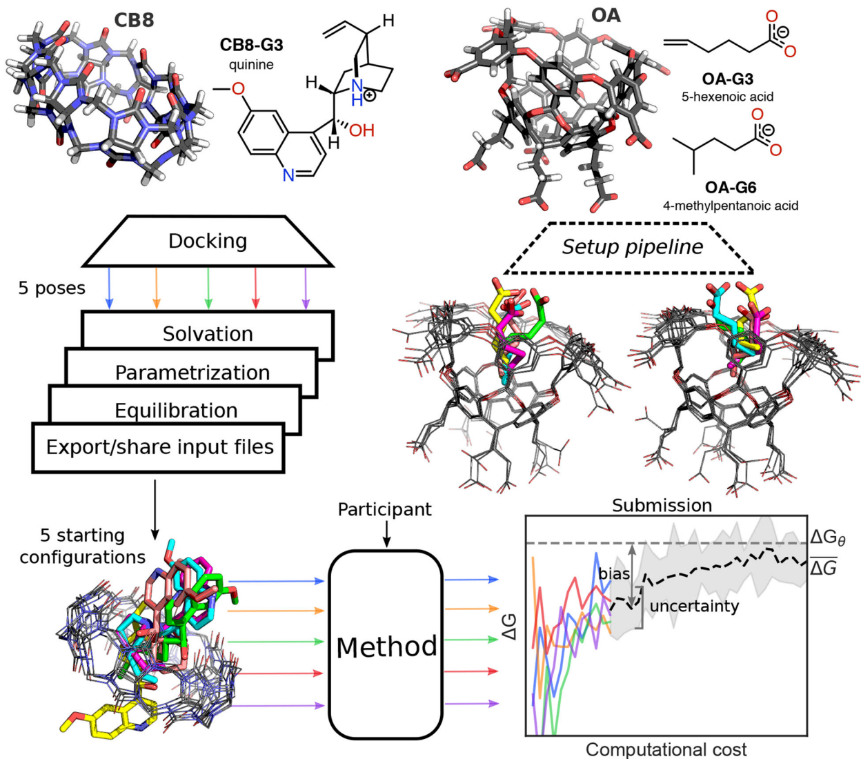
Figure 1. Challenge overview and initial conformations of the host-guest systems featured in the SAMPLing challenge.
