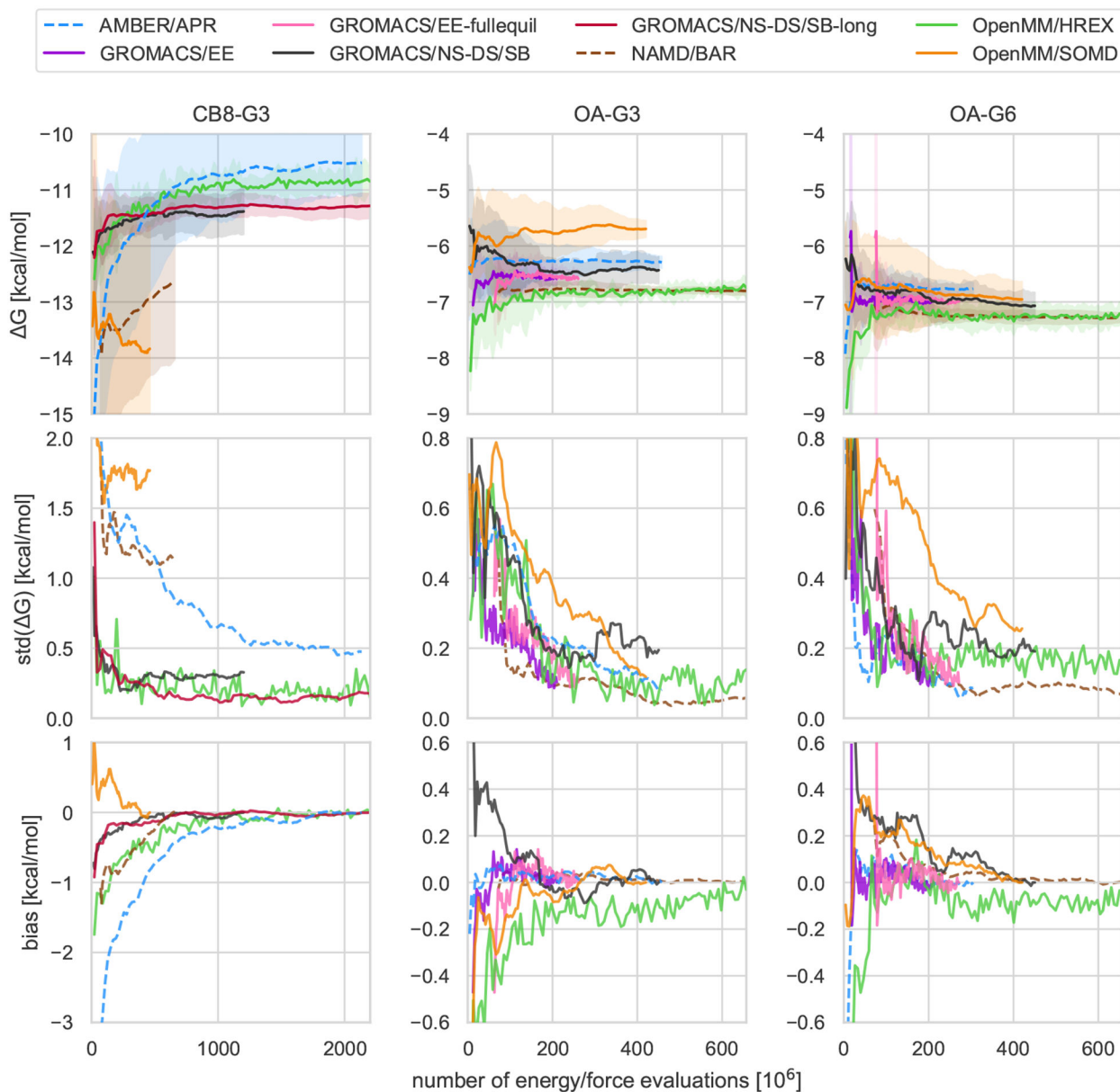
Figure 2. Mean free energy, standard deviation, and bias as a function of computational cost.
