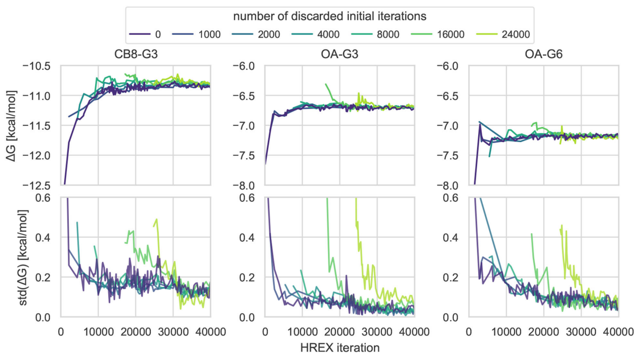
Figure 5. Initiating the HREX calculation from a single conformation introduces significant bias that slowly relaxes as the system reaches equilibrium.
