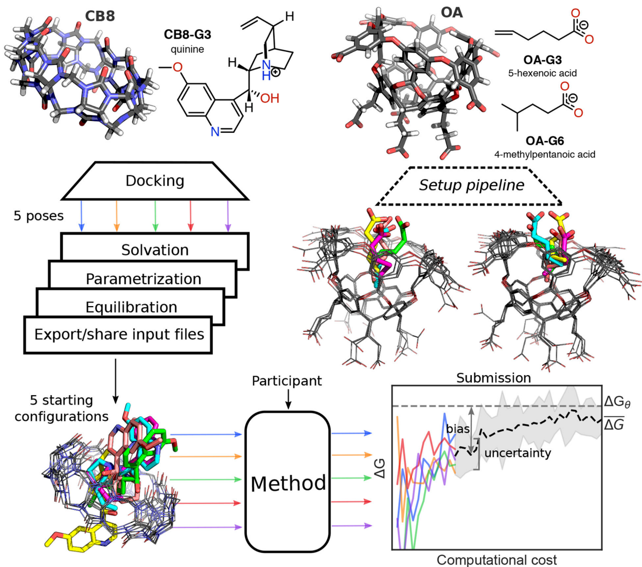
Figure 1. Challenge overview and initial conformations of the host-guest systems featured in the SAMPLing challenge.
