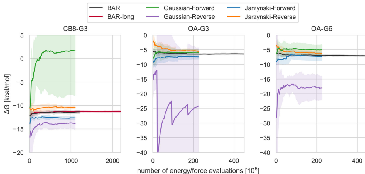
Figure 3. Comparison of bidirectional and unidirectional free energy estimators of the same nonequilibrium work switching data.
