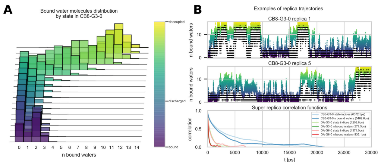
Figure 6. Bound water molecules induce metastability in HREX replicas with CB8-G3.
