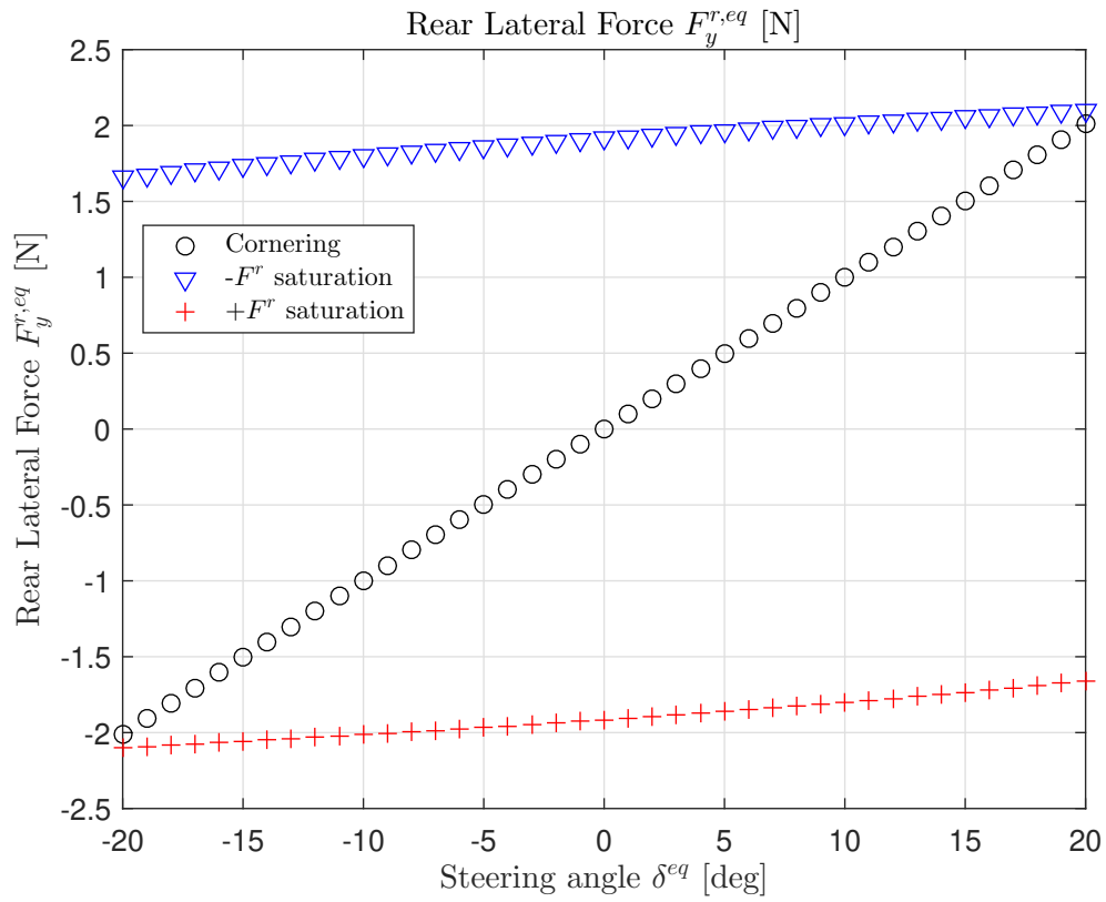
Figure 2.24: The rear lateral force F_y^{r,eq} scales linearly with the magnitude of the steering angle under typical cornering conditions (black circled curve). Under drift conditions (blue and red curves), the rear lateral force is saturated and shares the total available frictional force with the rear longitudinal force F_x^{r,eq} .
