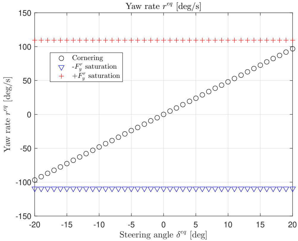
Figure 2.16: The yaw rate r scales linearly with the magnitude of the steering angle under typical cornering conditions (black circled curve). Under rear tire saturation (blue and red curves), the yaw rate maintains a large value.
