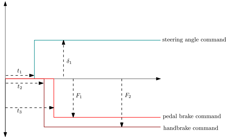
Figure 4.11: The control commands for aggressive maneuvers like drift roughly take the form of step functions that can easily be parameterized.
