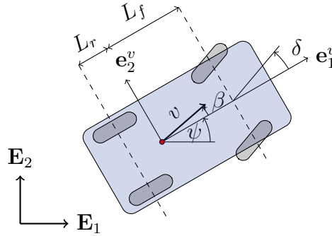
Figure 4.1: Vehicle model schematic
