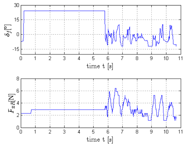
Figure 4.10: The RC state oscillates about the reference input.
