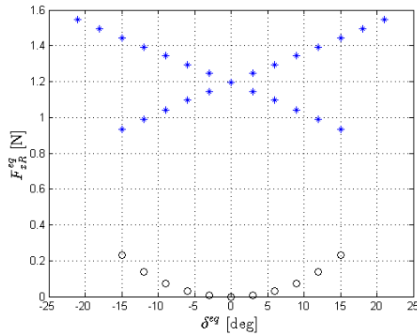
Figure 4.4: Equilibrium rear wheel force vs steering angle.
