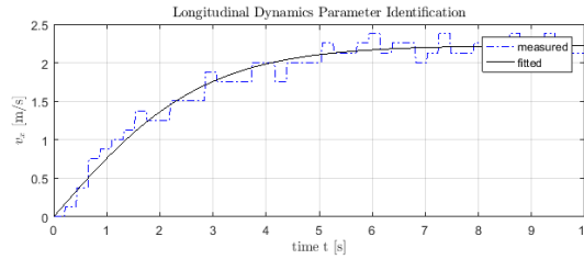
Figure 4.5: The optimized frictional and input gain parameters accurately longitudinal dynamics of the RC.
