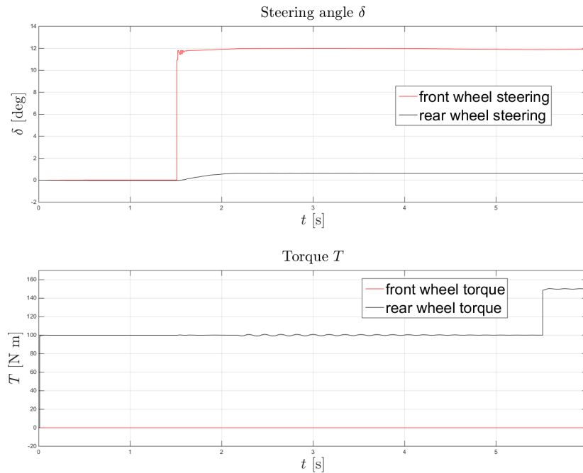
Figure 2.12: All system models initially drive straight and then turn to the left and apply a torque command to the motor.
