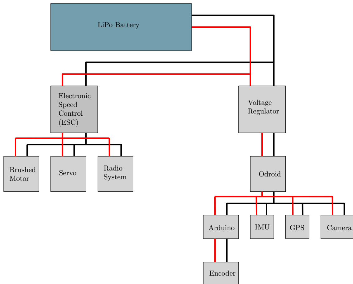
Figure 3.35: The Power distribution for BARC platform uses a single battery as the energy source.
