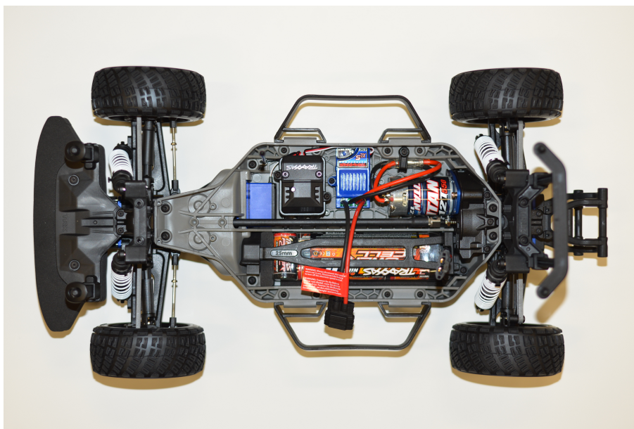
Figure 3.8: Top view of Traxxas Ford Fiesta ST Rally 1/10.
