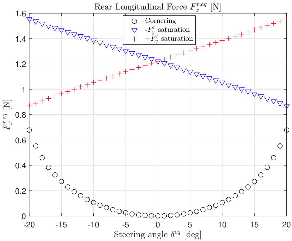
Figure 2.23: The rear longitudinal force F_x^r scales quadratically with the steering angle under cornering conditions. Under drift conditions (blue and red curves), the rear force takes the maximum value possible available from friction, which scales approximately linearly with the steering angle.
