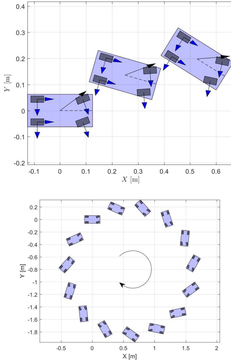
Figure 2.26: Top: The diagram shows the tire forces acting on the vehicle over three time steps. The blue arrows indicate the force vectors acting on each tire. The black arrow is the velocity vector, and the angle between the dashed line and the velocity vector is the slip angle \beta . Bottom: The bottom diagram shows the complete steady state motion of the vehicle. Equilibrium values: v_x^{eq} = 1.20 [m/s], \beta^{eq} = 36.63 [deg], r^{eq} = -79.99 [deg/s], \delta^{eq} = 20 [deg], F_x^{r,eq} = 1.5535 [N], F_y^{2r,eq} = -1.6587 [N].
