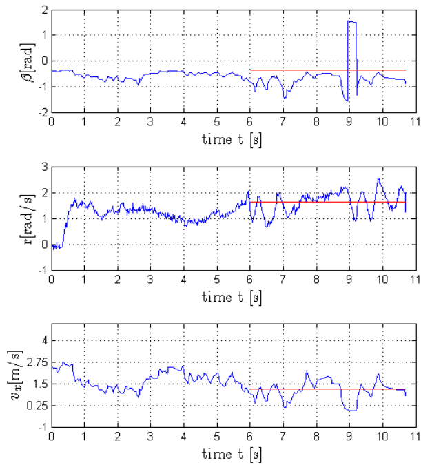
Figure 4.9: The RC state oscillates about the reference state.
