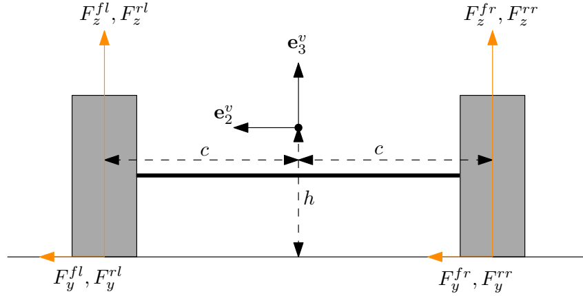
Figure 2.10: The lateral and vertical components of the tire forces acting within the \mathbf{e}_2^v - \mathbf{e}_3^v plane generate a moment about the \mathbf{e}_1^v axis. The positive \mathbf{e}_1^v axis points into the page (i.e., we are facing the rear side of the vehicle).
