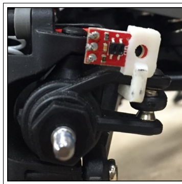
(b) Encoder mount
