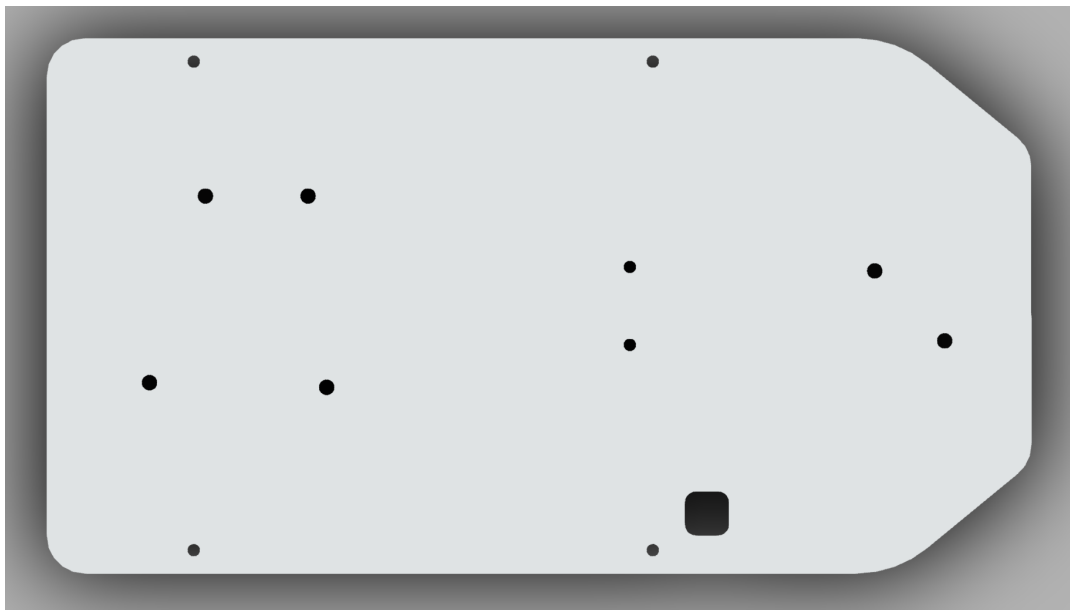
Figure 3.11: Top view of the BARC chassis base plate.
