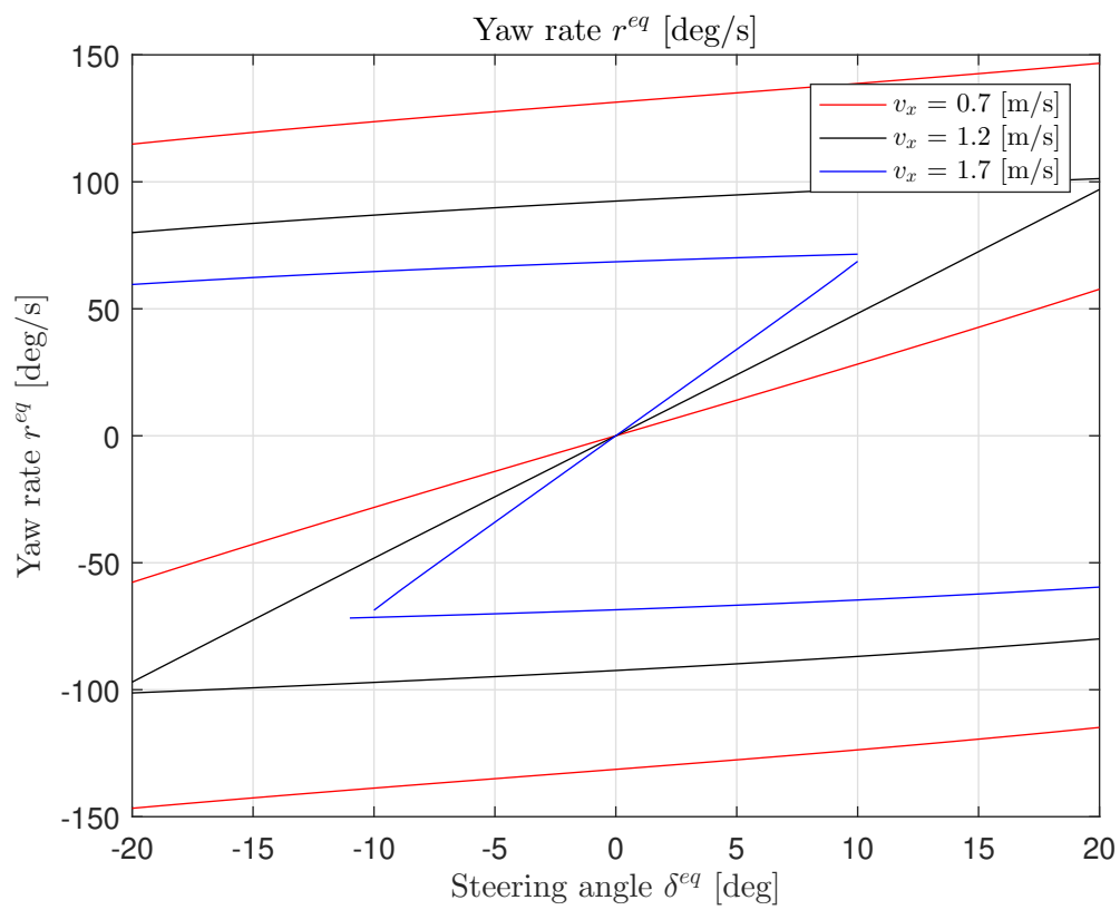
Figure 2.29: During drift conditions, the magnitude of the yaw rate r decreases as the magnitude of the longitudinal velocity increases for all steering angles.
