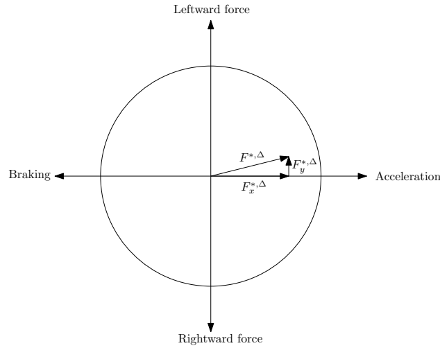
(a) During normal cornering, the vector sum of longitudinal and lateral components of the tire force lies within the limits of the friction circle.
