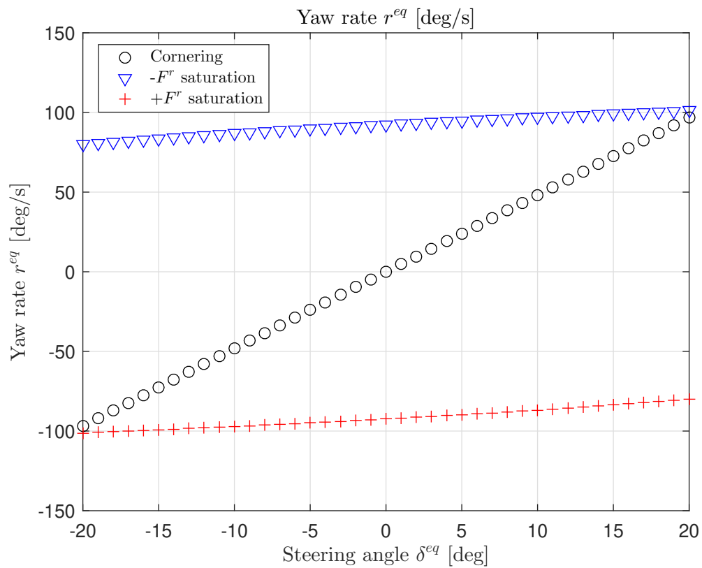
Figure 2.22: The yaw rate r scales linearly with the magnitude of the steering angle under typical cornering conditions (black circled curve). Under rear tire saturation (blue and red curves), the yaw rate maintains a large value.
