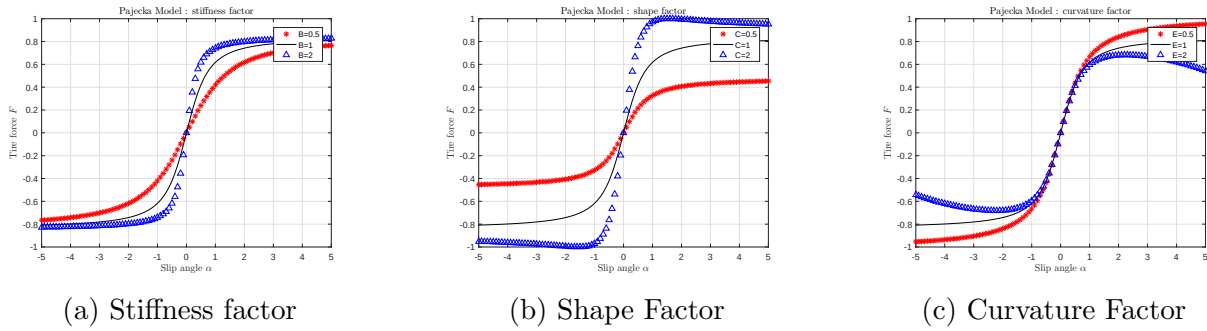
Figure 2.7: The Pacejka tire model is characterized by coefficients that manipulate different properties of the force curve, such as amplitude, curvature, and tail behavior.
