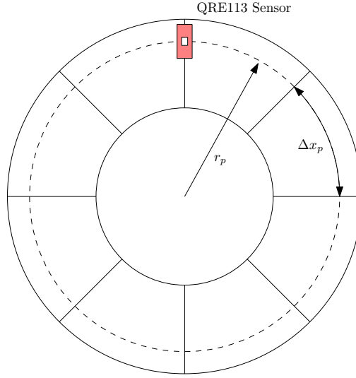
Figure 3.14: Velocity is computed by counting the number of switches between light and dark partition over a fixed time interval, and then using geometric information of the encoder unit.
