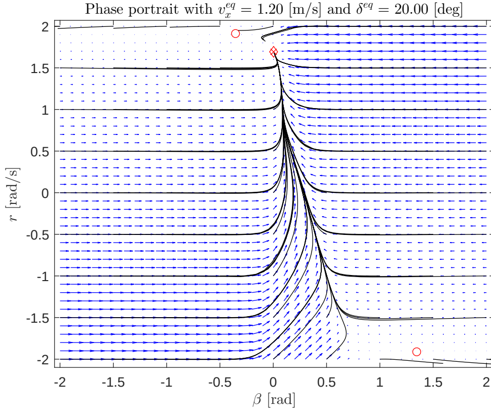
Figure 2.20: The phase portrait illustrates three equilibria associated with the vehicle running at v_x = 1.20 [m/s] and \delta^{eq} = +20.00 [deg]. The small, open, red circles at the top and bottom of the plot indicate unstable drift equilibrium, and the diamond shaped red marker around at around (\beta = 0.00, r = 1.69) indicates a stable equilibrium, or normal cornering condition. The black lines and blue arrows indicate fields or how the system starting at any state within the space shown would evolve. As expected, the system moves toward the stable equilibrium state.
