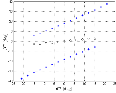
Figure 4.2: Equilibrium sideslip angle vs steering angle
