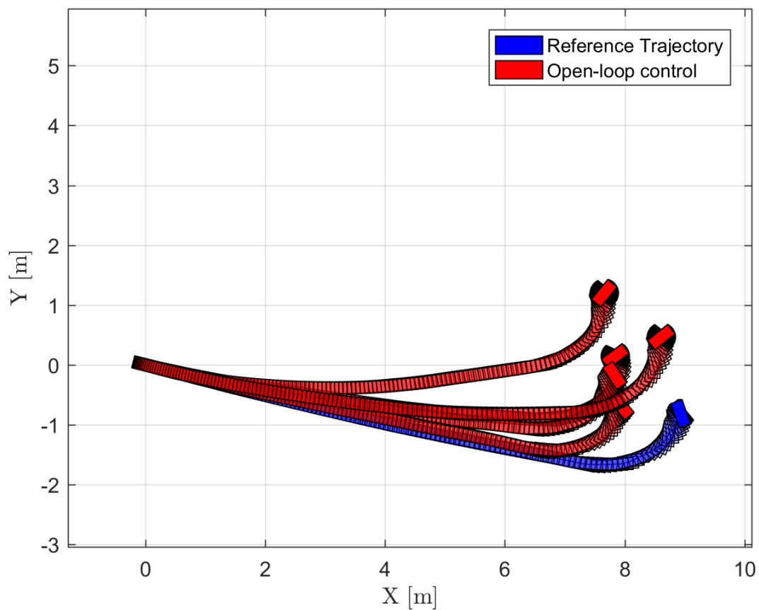
Figure 4.14: Applying a pure open-loop controller over a long time horizon fails to track the reference trajectory. The blue trajectory denotes the reference trajectory and the red trajectories are all experimental results from applying the same control inputs as the reference trajectory in open-loop.
