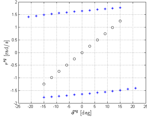
Figure 4.3: Equilibrium yaw rate vs steering angle.
