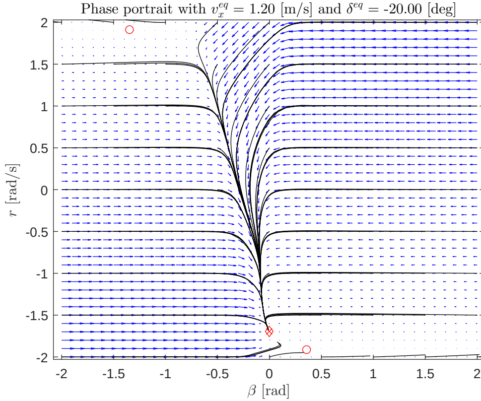
Figure 2.19: The phase portrait illustrates three equilibria associated with the vehicle running at v_x = 1.20 [m/s] and \delta^{eq} = -20.00 [deg]. The small, open, red circles at the top and bottom of the plot indicate unstable drift equilibrium, and the diamond-shaped red marker around at around (\beta = 0.04, r = -1.77) indicates a stable equilibrium, or normal cornering condition. The black lines and blue arrows indicate fields or how the system starting at any state within the space shown would evolve. As expected, all systems would move toward the stable equilibrium state.
