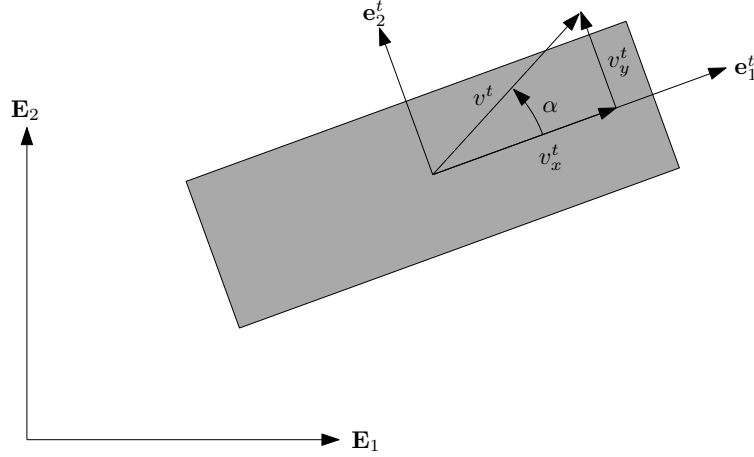
Figure 2.3: The tire side slip measures the angle between the lateral and longitudinal component of the tire velocity vector.
