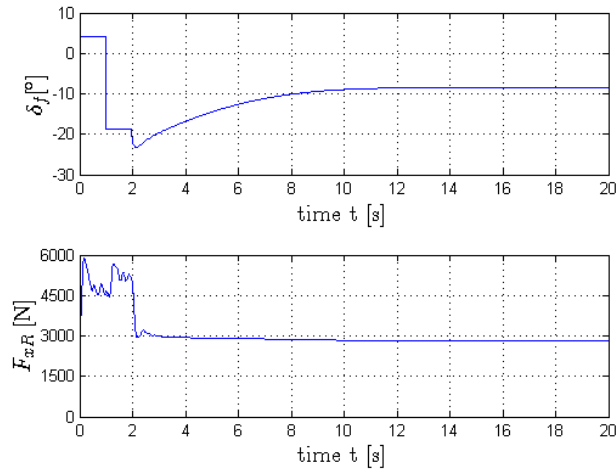
Figure 4.8: The CarSim vehicle input converges to the reference input.
