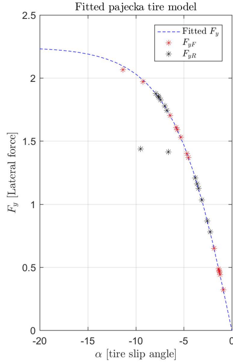
Figure 4.6: The optimized tire model parameters from program (4.10) fit the experimental data. The red and black asterisks represent tire forces estimated directly from data using the dynamic equations, and the dashed blue line comes from the tire model with optimized parameters and slip-angle estimates from data
