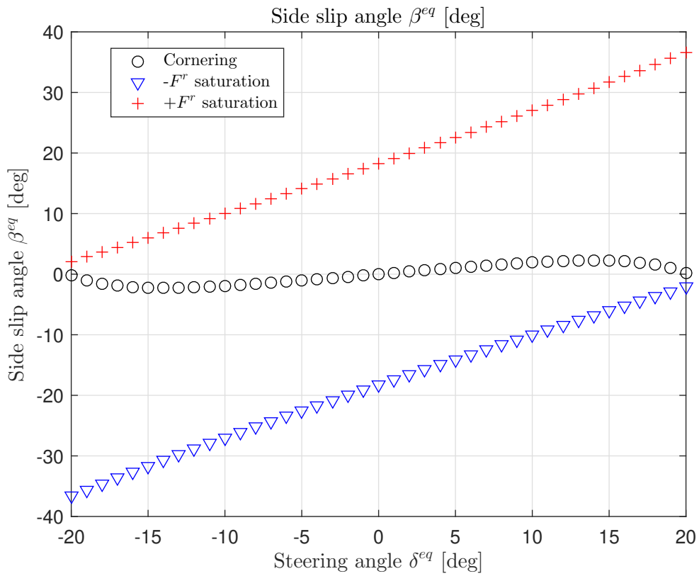
Figure 2.21: The side slip angle \beta does not grow beyond a couple of degrees under normal cornering conditions (black circled curve). Under rear tire saturation (blue and red curves), the slip angles grow to a large value.
