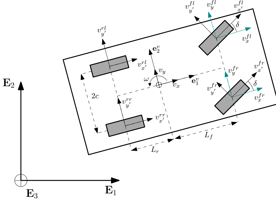
Figure 2.4: Longitudinal and lateral components of tire velocity in a four-wheel vehicle model.
