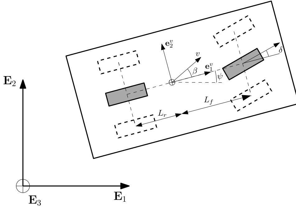
Figure 2.2: Kinematic Bicycle Model.
