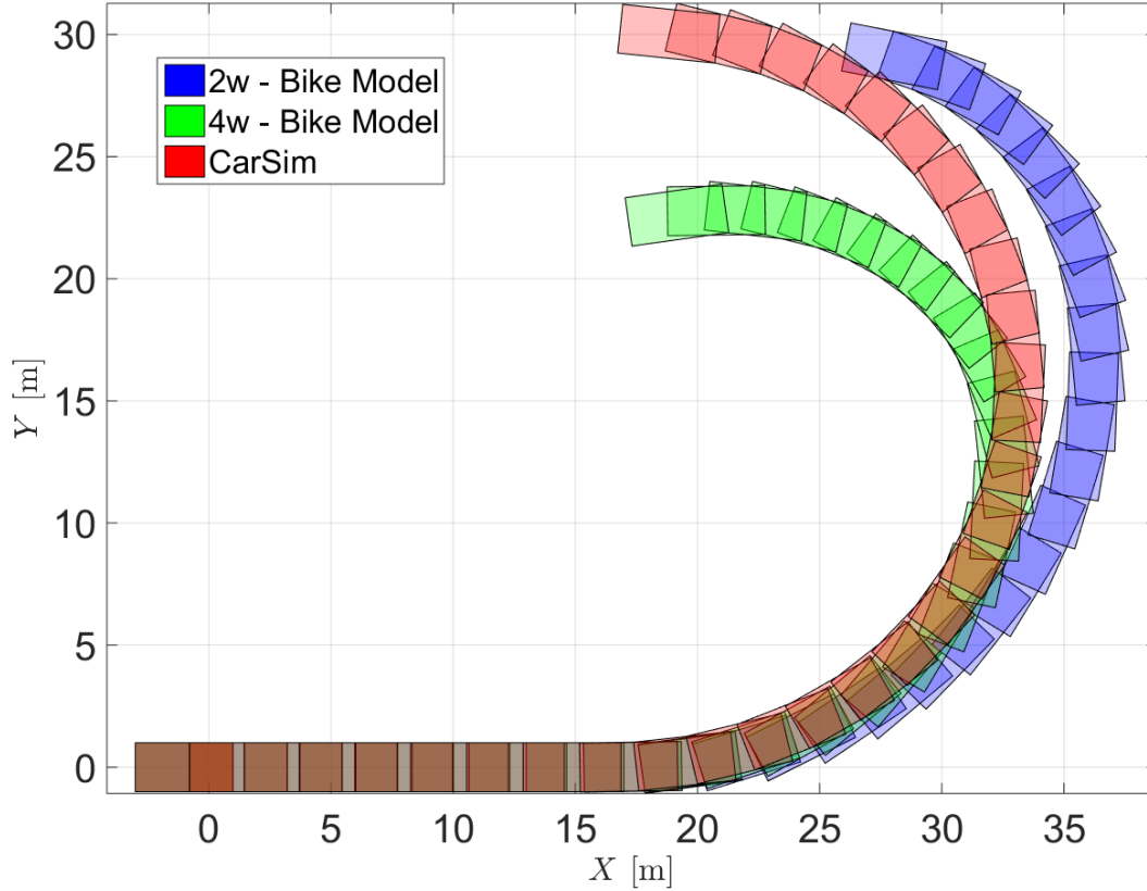
Figure 2.13: The trajectories from the two-wheel (blue) and four-wheel (green) models both diverge from the trajectory of the CarSim model (red) as the vehicle enters into the drift maneuver.
