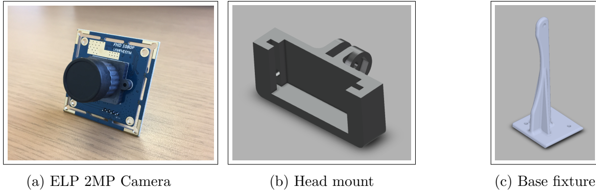
Figure 3.17: The ELP 2MP Monocular Camera can deliver 280 x 720 P images at 60 fps
