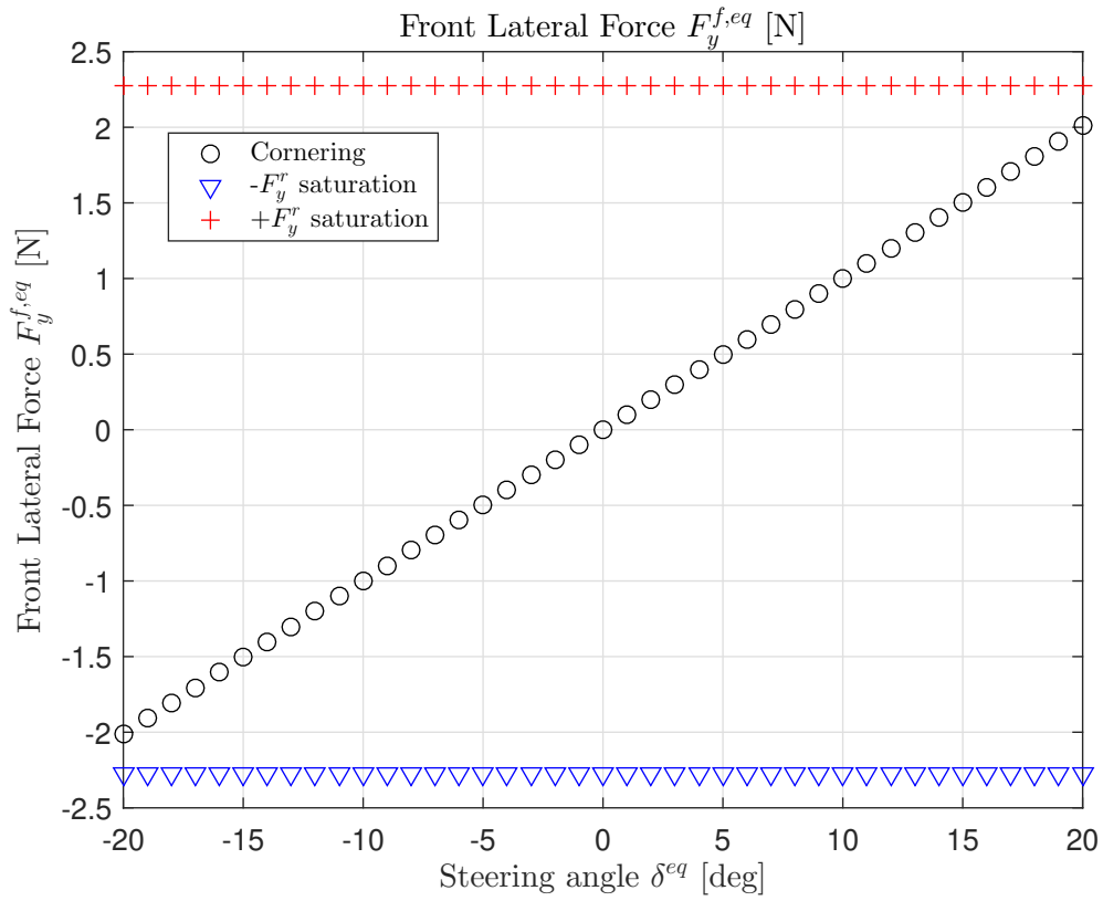
Figure 2.17: The front lateral force F_y^{f,eq} scales linearly with the magnitude of the steering angle under typical cornering conditions (black circled curve). Under drift conditions (blue and red curves), the rear lateral force is saturated and the front lateral force maintains a large value.
