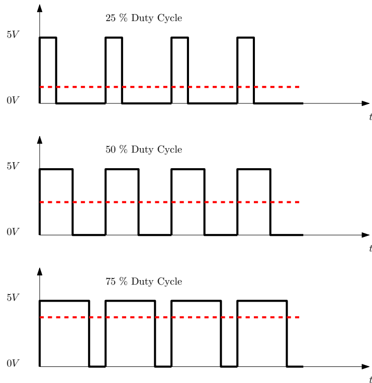
Figure 3.10: Pulse Width Modulation can encode information or control power delivered to electrical devices. From top to bottom, the PWM curves illustrate 25%, 50%, and 75% duty cycles, respectively. The red dashed line shows the average voltage value over the cycle. A higher duty cycle means more power is delivered to connected devices.
