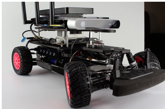
Figure 3.3: The RACECAR is an open-source platform from MIT. Image from [27]
