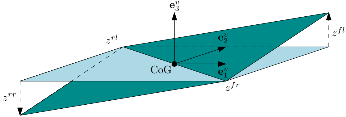
Figure 2.11: The vertical deformation of the tires are balanced in the diagonal direction.
