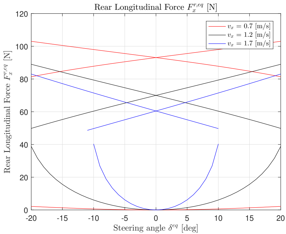
Figure 2.30: During drift conditions, the magnitude of the rear longitudinal force F_x^r decreases as the magnitude of the longitudinal velocity increases for all steering angles.
