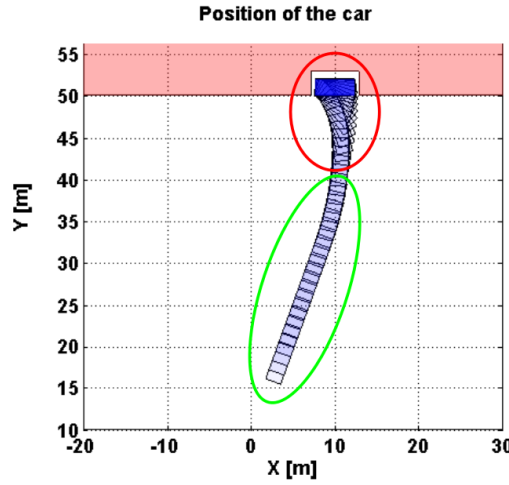
Figure 4.12: The vehicle has a low side-slip angle in the highlighted green segment and a high-slip angle in the red segment.
