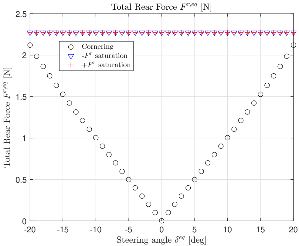
Figure 2.25: The total rear force under cornering conditions scales approximately linearly with the steering angle. This result makes sense as the lateral force operates in the linear region of the tire model. Under drift conditions (blue and red curves), the rear tires are saturated for all steering angles, which results in the straight horizontal line at the top at value (\mu F_z^r) .
