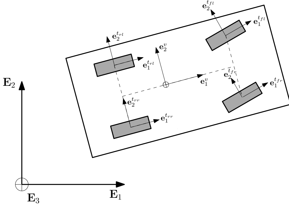
Figure 2.1: Coordinate system for vehicle motion.
