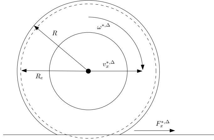
Figure 2.5: The slip-ratio measures the amount of deformation along the rolling direction of the tire.
