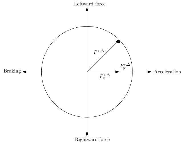
(b) During tire saturation, the vector sum of longitudinal and lateral components of the tire force reach the limits of the friction circle.
