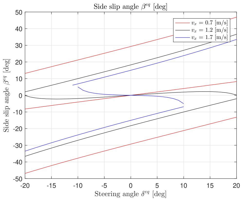
Figure 2.28: During drift conditions, the magnitude of the side slip angle \beta decreases as the magnitude of the longitudinal velocity increases for all steering angles.
