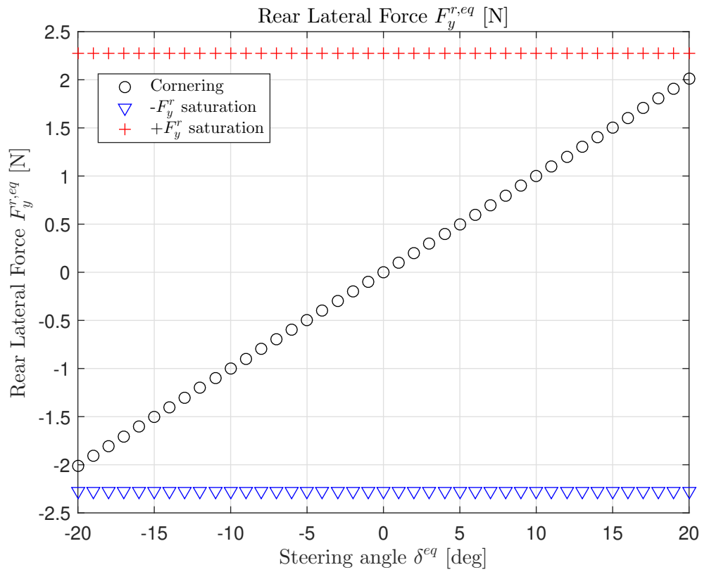
Figure 2.18: The rear lateral force F_y^{r,eq} scales linearly with the magnitude of the steering angle under typical cornering conditions (black circled curve). Under drift conditions (blue and red curves), the rear lateral force is saturated.
