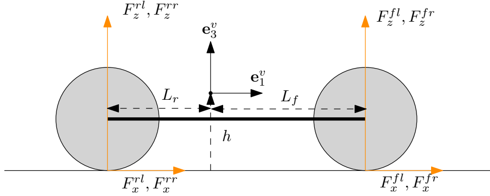
Figure 2.9: The longitudinal and vertical components of the tire forces acting within the \mathbf{e}_1^v - \mathbf{e}_3^v plane generate a moment about the \mathbf{e}_2^v axis. The positive \mathbf{e}_2^v axis points into the page
