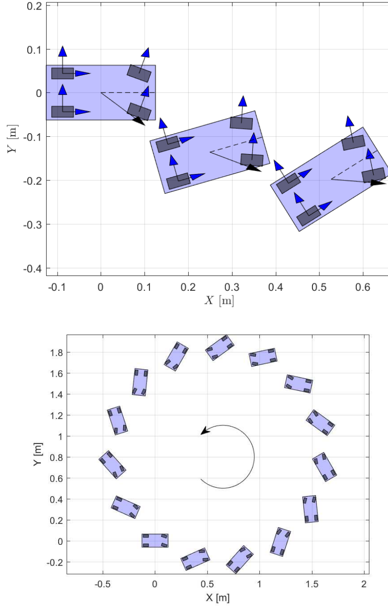
Figure 2.27: Top: The diagram shows the tire forces acting on the vehicle over three time steps. The black arrow is the velocity vector, and the angle between the dashed line and the velocity vector is the slip angle \beta . Bottom: The bottom diagram shows the complete steady state motion of the vehicle. Equilibrium values: v_x^{eq} = 1.20 [m/s], \beta^{eq} = -36.63 [deg], r^{eq} = 79.99 [deg/s], \delta^{eq} = -20 [deg], F_x^{r,eq} = 1.5535 [N], F_y^{r,eq} = 1.6587 [N]. The equilibrium state represents a mirror opposite of the state in Figure 2.26.
