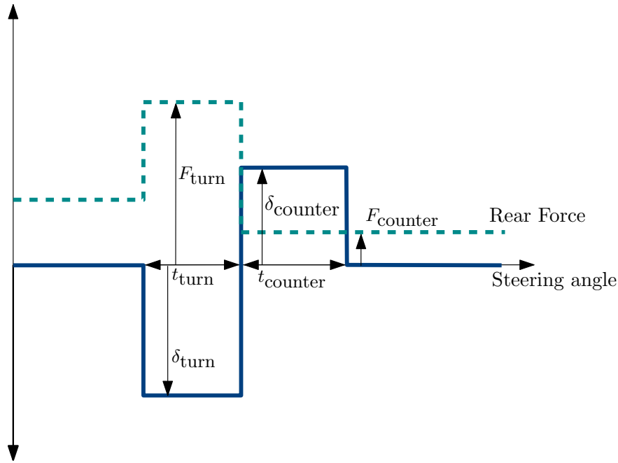
Figure 4.16: Parametrized control sequence for drift cornering
