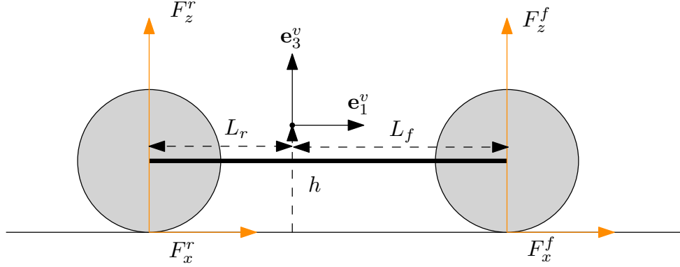
Figure 2.8: The longitudinal and vertical components of the tire forces acting within the \mathbf{e}_1^v - \mathbf{e}_3^v plane generate a moment about the \mathbf{e}_2^v axis. The positive \mathbf{e}_2^v axis points into the page.
