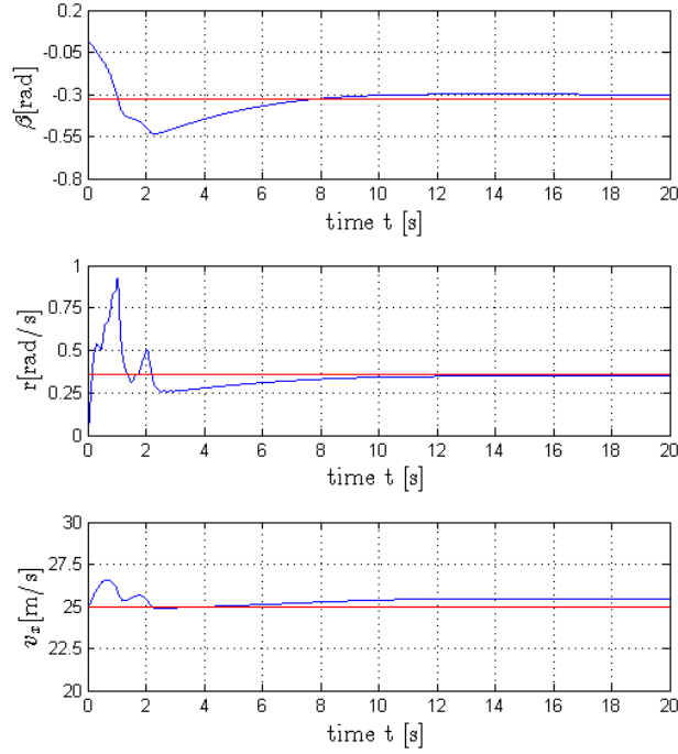
Figure 4.7: The CarSim vehicle state converges to the reference state.
