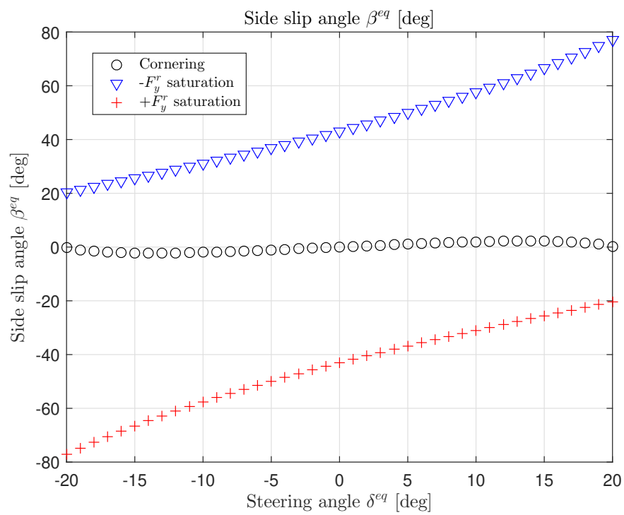
Figure 2.15: The side slip angle \beta does not grow beyond a couple of degrees under normal cornering conditions (black circled curve). Under rear tire saturation (blue and red curves), the slip angles grow to large values.
