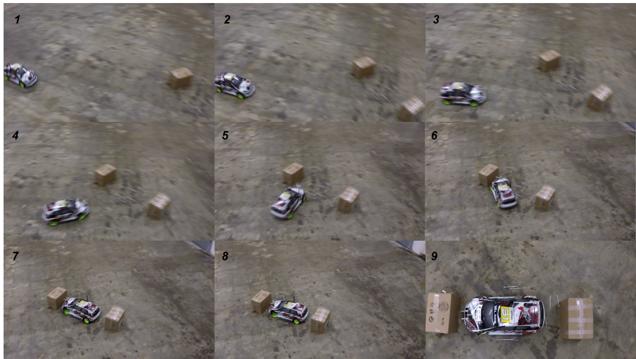
Figure 4.15: The frame-by-frame image shows the vehicles approaching, turning, and then sliding into the parking spot between the boards during an experimental run.
