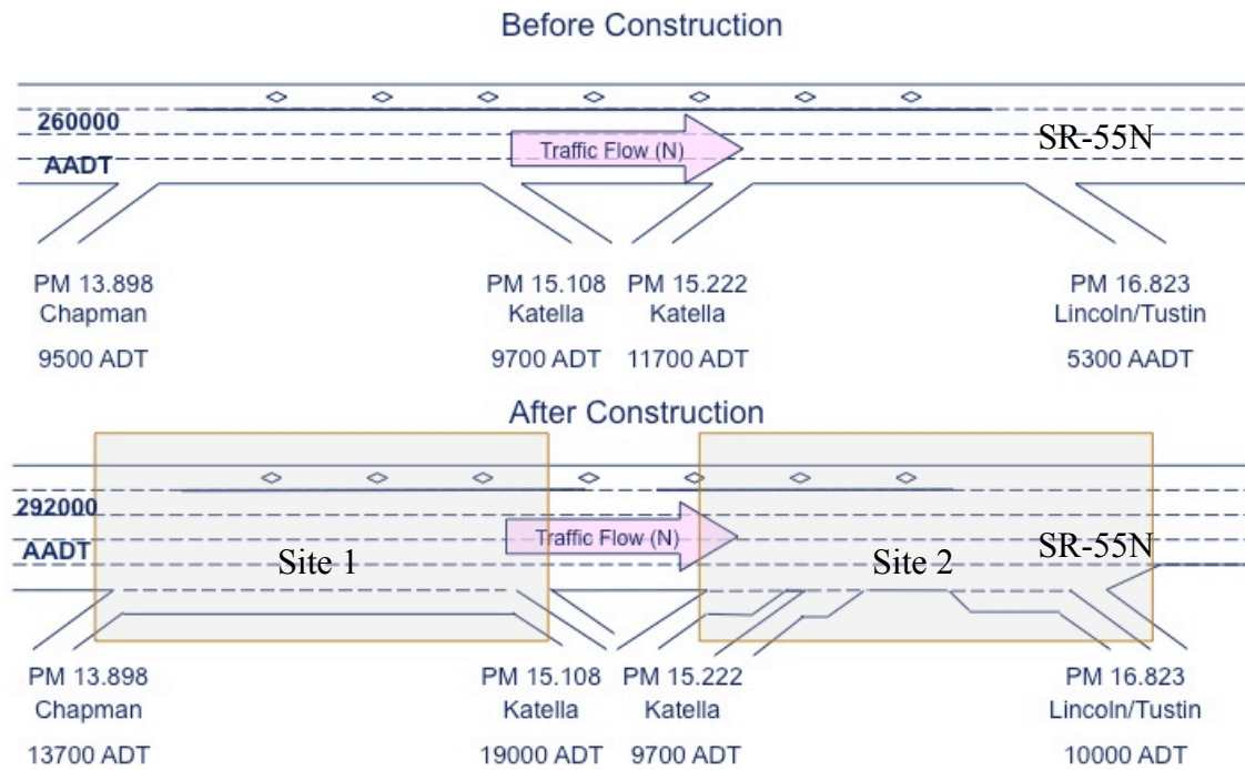
Figure 3. Geometric configuration of study sites 1 and 2
