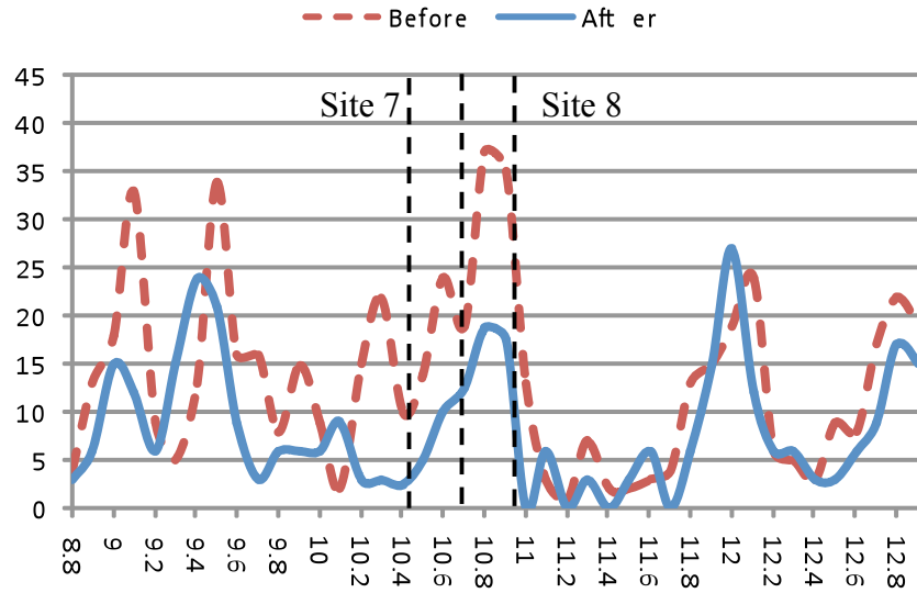
Figure 13. Collision profile of study sites 7 and 8
