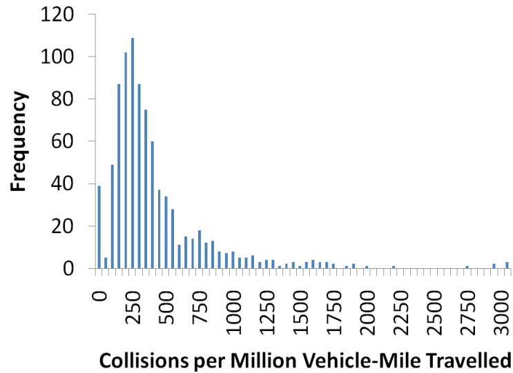
Figure 18. Southbound, ramps & 4000 ft. up/downstream
