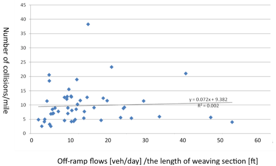
Figure 27. Collision rate vs. off-ramp flow/weaving section length
