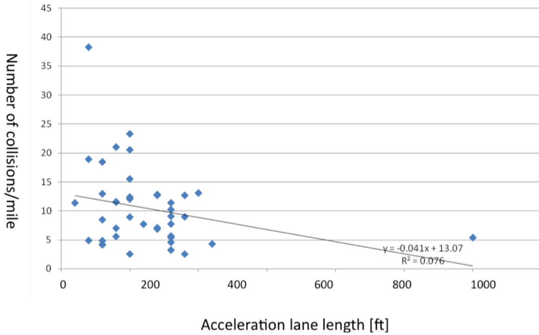
Figure 28. Collision rate vs. acceleration lane length
