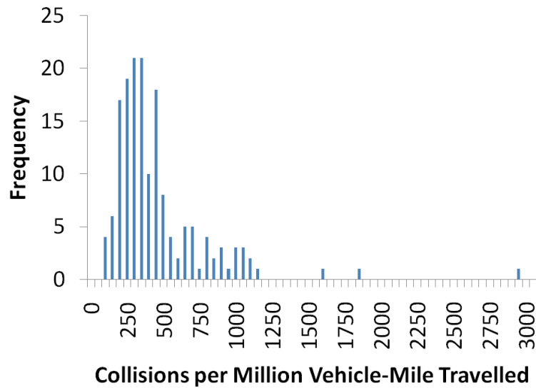
Figure 20. Southbound, weaving sections & 4000 ft. up/downstream
