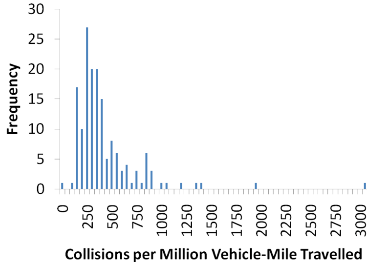
Figure 19. Northbound, weaving sections & 4000 ft. up/downstream
