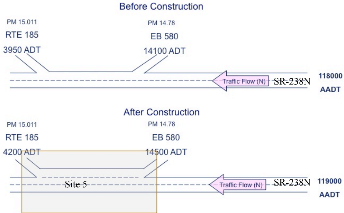
Figure 5. Geometric configuration of study site 5
