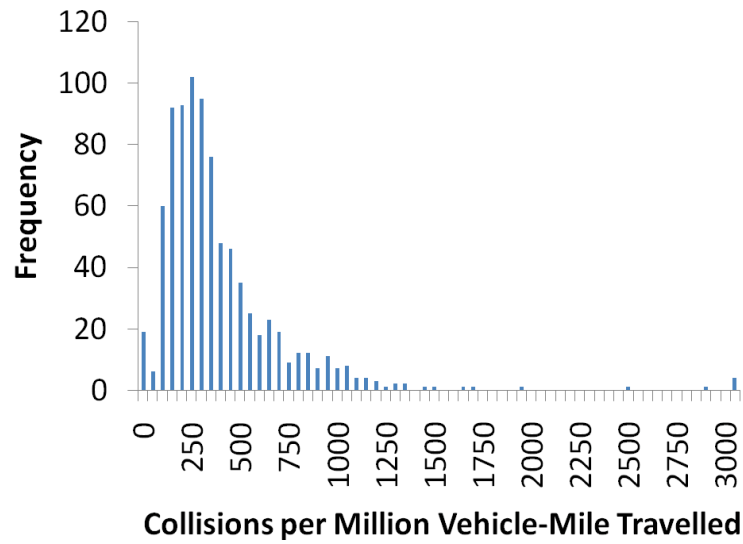
Figure 17. Northbound, ramps & 4000 ft. up/downstream
