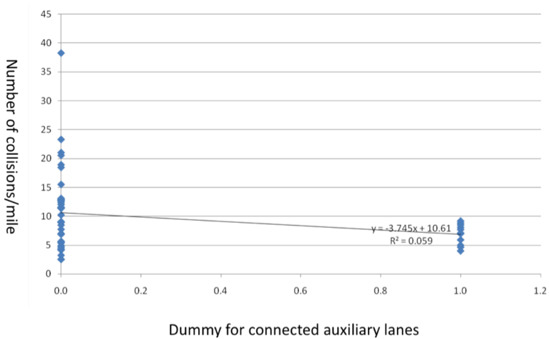
Figure 30. Collision rate vs. dummy variable for connected auxiliary lanes (1=auxiliary lanes; 0=no auxiliary lanes)
