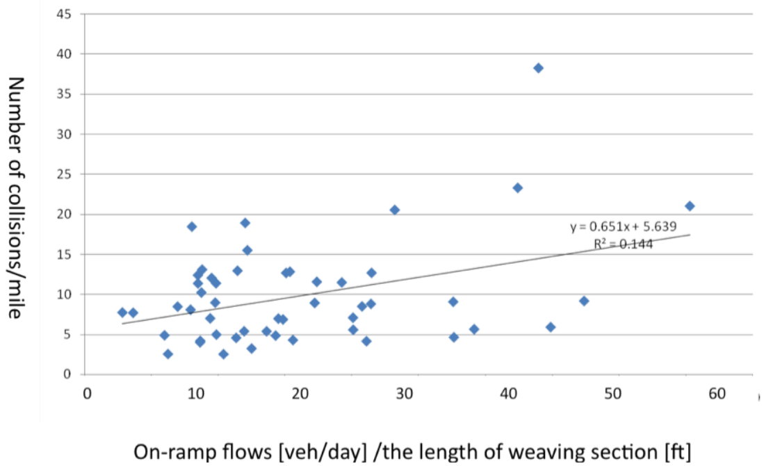
Figure 25. Collision rate vs. on-ramp flow/weaving-section length
