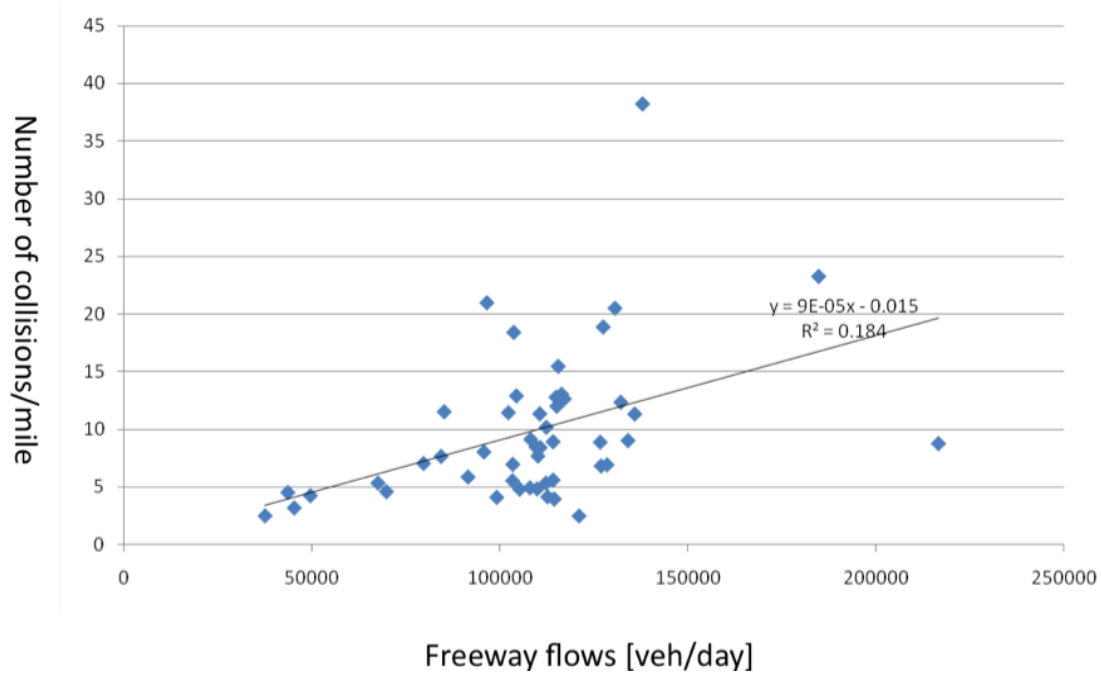
Figure 23. Collision rate vs. freeway flow
