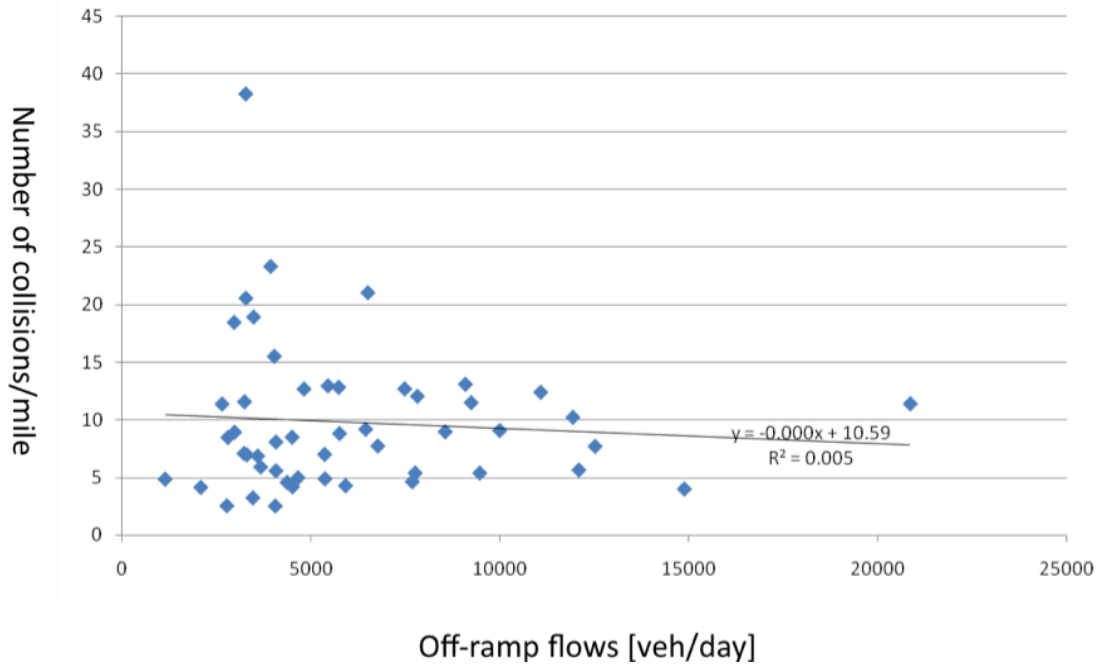
Figure 26. Collision rate vs. off-ramp flow
