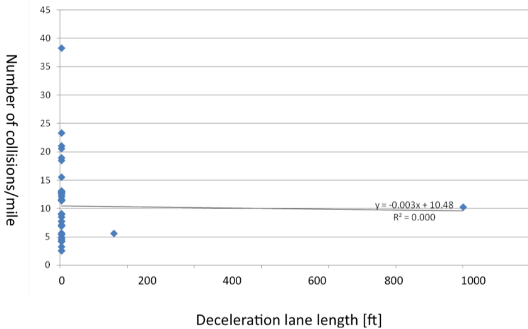
Figure 29. Collision rate vs. deceleration lane length
