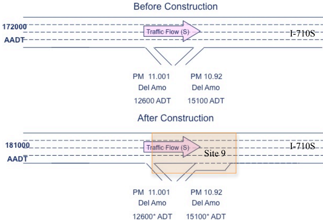
Figure 15. Geometric configuration of study site 9
