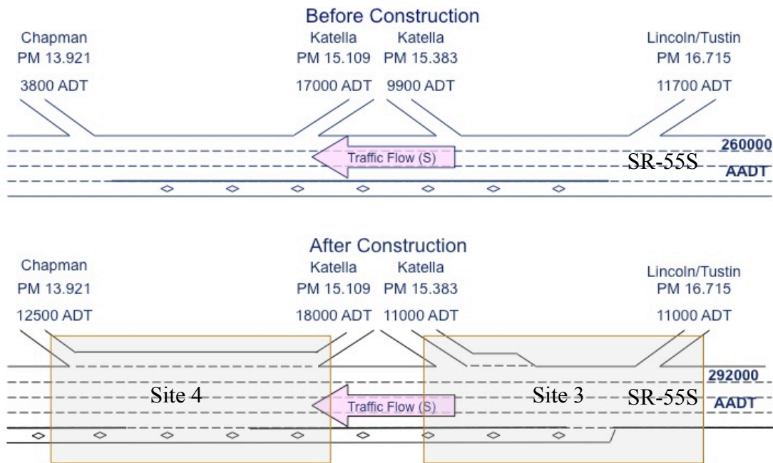
Figure 5. Geometric configuration of study sites 3 and 4
