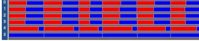
Fig. 7. States of six unbalanced tasks on a network of workstations.
