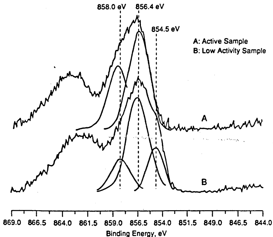
Fig. 4. \text{Ni}_{2p_{3/2}} XPS spectra from an active (A) and a low activity (B) Ca/Ni/K-2:1:0.1 oxide catalyst.
