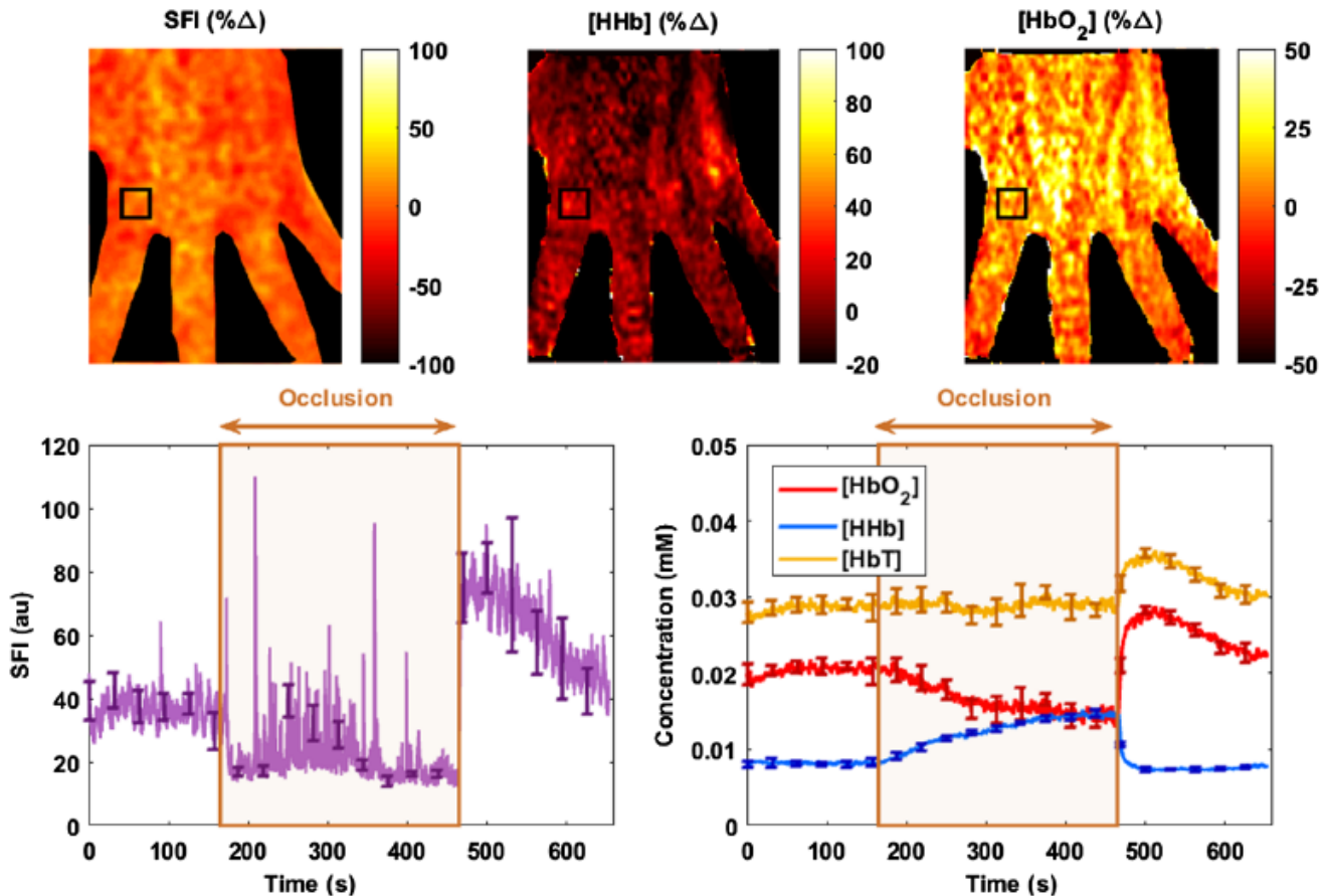
Fig. 8 Still image from a video of dynamic changes during an arterial occlusion and reperfusion challenge. The images from left to right depict maps of percent change of SFI, [HHb], and HbO 2 , respectively. The bottom-left plot shows time-series SFI in arbitrary units versus time in seconds. The bottom-right plot shows time-series [HbT], HbO 2 , and [HHb] in yellow, red, and blue, respectively. (Video 1, QuickTime, 11.4 MB [URL: https://doi.org/10.1117/1.JBO.23.3.036013.1 ]).
