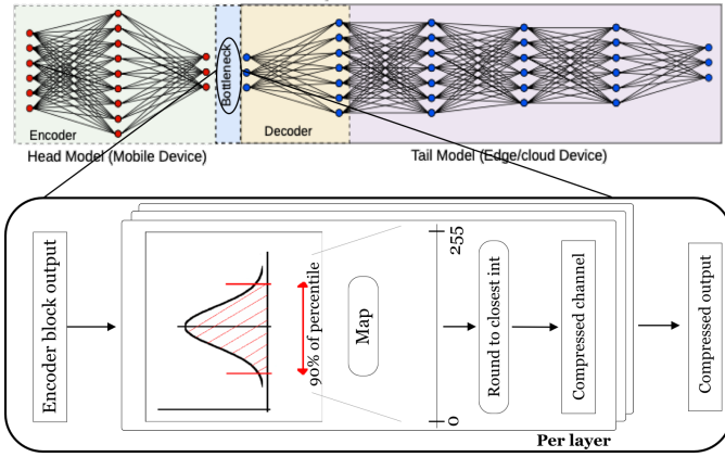
Fig. 3. Saturation Quantizer truncated quantization process.
