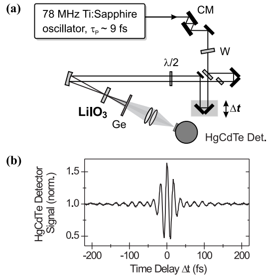
Fig. 1. (a) Oscillator-based setup for THz pulse generation in \text{LiIO}_3 and for interferometric field correlations. W: 1-mm thick fused-silica window, CM: chirped mirrors with \approx -200 \text{ fs}^2 group delay dispersion, Ge: Germanium window. (b) interferogram generated with a 113\text{-}\mu\text{m} thick crystal near normal incidence.
