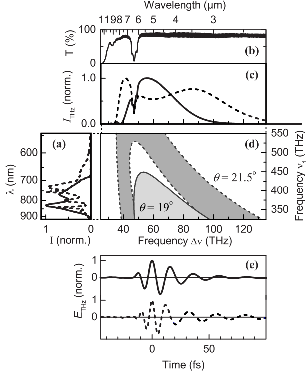
Fig. 3. (a) Spectra of 9-fs Ti:sapphire oscillator pulses (solid line) and of 7-fs pulses from a hollow fiber compressor, HFC (dashed). (b) normal incidence transmission of 113- \mu\text{m} thick \text{LiIO}_3 . (c)-(e) Calculations of phase-matched difference frequency mixing in this crystal. Results are for \theta = 19^\circ pumped by the oscillator (solid lines), and for \theta = 21.5^\circ pumped by the HFC (dashed): (c) THz spectra, (d) frequency space (shaded) with L_C > 100 \mu\text{m} , (e) time-domain THz electric fields.
