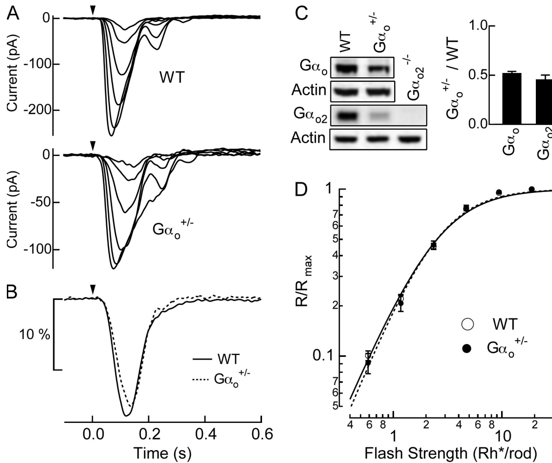
Figure 4. Reduced G\alpha_o expression in G\alpha_o^{+/-} mice does not alter rod bipolar responses (A) Responses to a family of flashes producing 0.59, 1.2, 2.4, 4.7, 9.4, and 19 Rh*/rod were recorded in a WT ( G\alpha_o^{+/+} littermate), and a G\alpha_o^{+/-} rod bipolar cell. (B) Normalized rod bipolar response to dim flashes producing 1 Rh*/rod was estimated by averaging normalized responses to dim flashes causing 5–25% of maximal responses and dividing it by the average dim flash strength, which was 0.73 Rh*/rod for WT and 0.79 Rh*/rod for G\alpha_o^{+/-} . The WT response is the average of 437 dim flash responses across 14 cells from 3 mice, and the G\alpha_o^{+/-} response is the average of 271 dim flash responses across 15 cells from 3 mice. (C) The total amount of G\alpha_o and G\alpha_{o2} proteins in WT and G\alpha_o^{+/-} retinas were compared using Western blot analysis. The amount of G\alpha_{o2} proteins in G\alpha_{o2}^{-/-} retinas was also examined to check the specificity of the antibody. The protein level of G\alpha_o^{+/-} retina was normalized to that of WT retina for a pair of WT and G\alpha_o^{+/-} mice used in one experiment, and the collected results are shown in the bar graph. The error bars are the SEM. The G\alpha_o protein levels were 1 vs. 0.52 \pm 0.02 ( n = 4 ) and the G\alpha_{o2} protein levels were 1 vs. 0.46 \pm 0.04 ( n = 3 ) (mean \pm SEM, WT vs. G\alpha_o^{+/-} ). (D) Normalized response amplitudes from individual families were averaged across cells for WT rod bipolar cells ( n = 14 ) and G\alpha_o^{+/-} rod bipolar cells ( n = 15 ) and plotted as a function of flash strength. Half-maximal flash strengths estimated from the Hill curve fits were 2.5 \pm 0.13 vs. 2.5 \pm 0.17 Rh*/rod, and the Hill exponents were 1.54 \pm 0.04 vs. 1.62 \pm 0.06 (mean \pm SEM, WT vs. G\alpha_o^{+/-} ).
