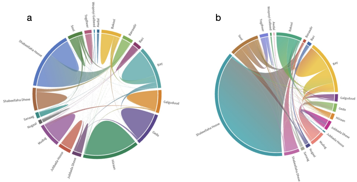
Figure 3.2: Circos diagram of total internal displacements between regions in Somalia from 2016 to 2023 where (a) represents all migration flows and (b) leaves out the flows that occurred within the same region.
