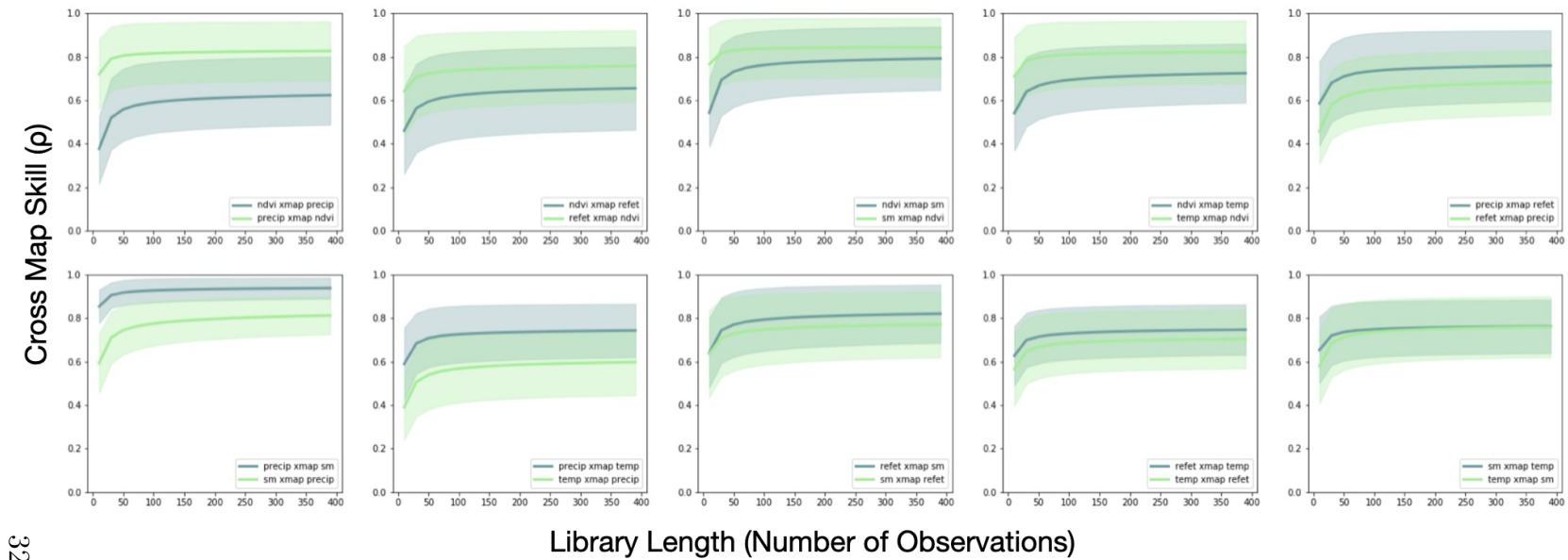
Figure 2.8: Cross mappings between each set of variable pairs (combinations of NDVI, precipitation, refET, soil moisture, and LST) across all cropland pixels in East Africa. Skill is measured by the Pearson’s correlation coefficient ( \rho ) of the estimated and observed values of the target variable (e.g., in the first panel, the blue line ‘ndvi xmap precip’ means that NDVI is the candidate manifold cross-mapping onto the target, precipitation). Solid lines are the average cross-map skill for all pixels, and shaded areas show the range of results for all pixels. The two sets converge rapidly in each subplot, indicative of bidirectional causation. The gap in average lines can be interpreted as the relative strength of one variable forcing another. For instance, in the first panel, precipitation wields a strong effect on NDVI based on the relatively large vertical separation between the two compared to other combinations, particularly that of soil moisture and temperature, where the lines are nearly indistinguishable, suggestive of nearly identical historical signatures or immediate feedbacks.
